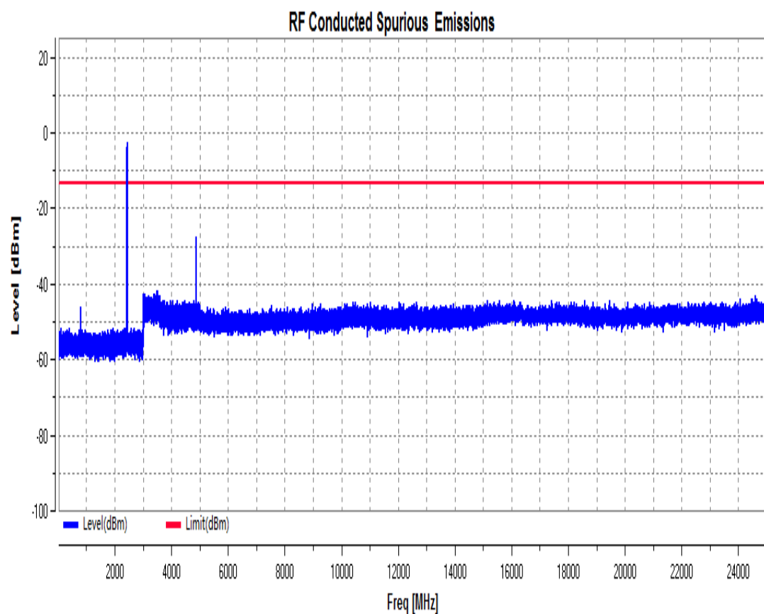
RF Conducted Spurious Emissions_11B_2437_Ant1
