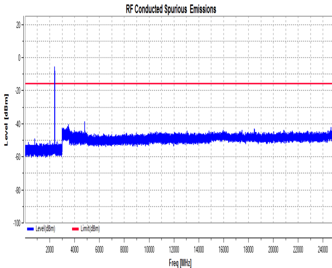
RF Conducted Spurious Emissions_11G_2412_Ant2
