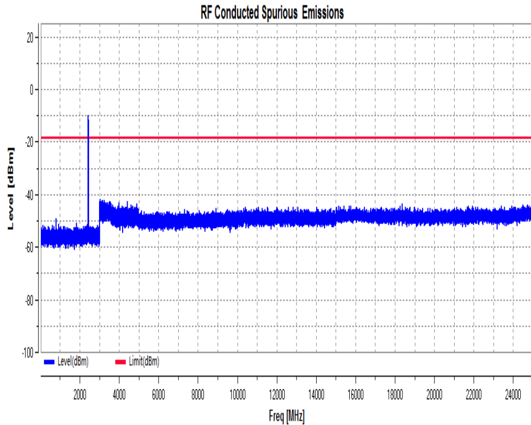
RF Conducted Spurious Emissions_11N40MIMO_2437_Ant1+2
