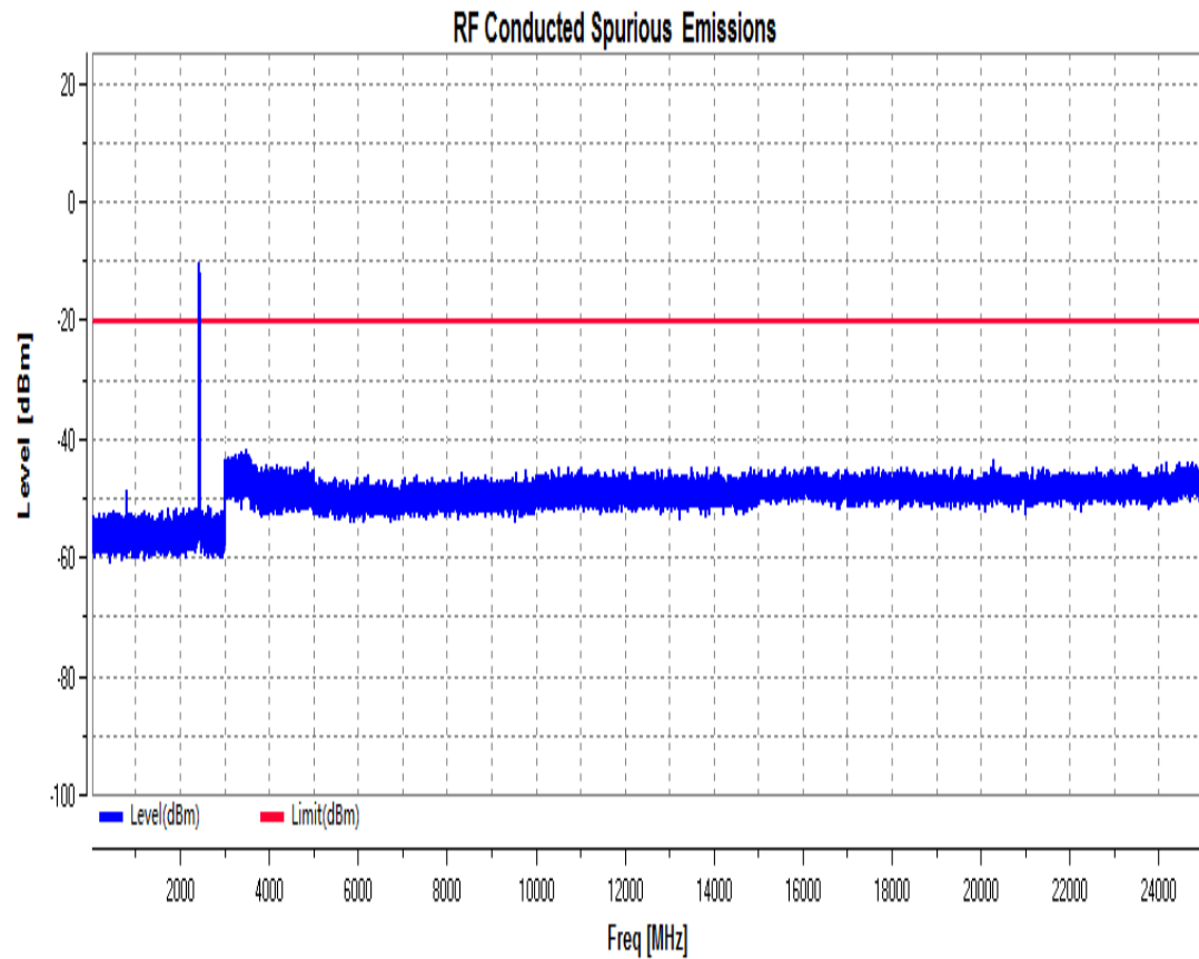
RF Conducted Spurious Emissions_11N40SISO_2437_Ant2
