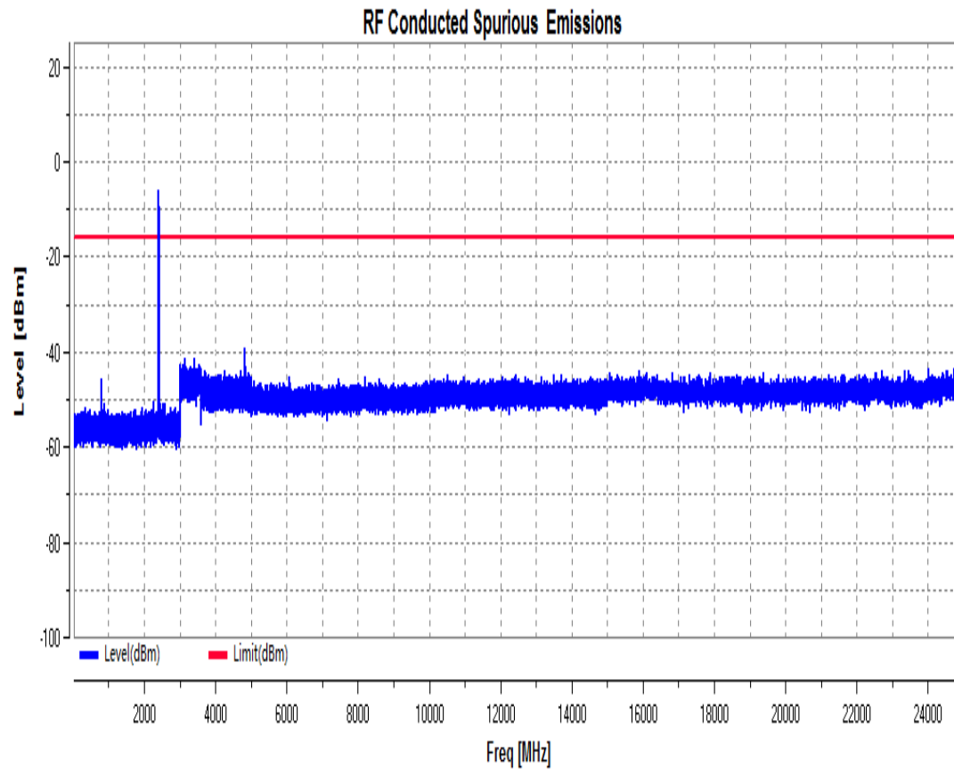
RF Conducted Spurious Emissions_11N20SISO_2412_Ant1
