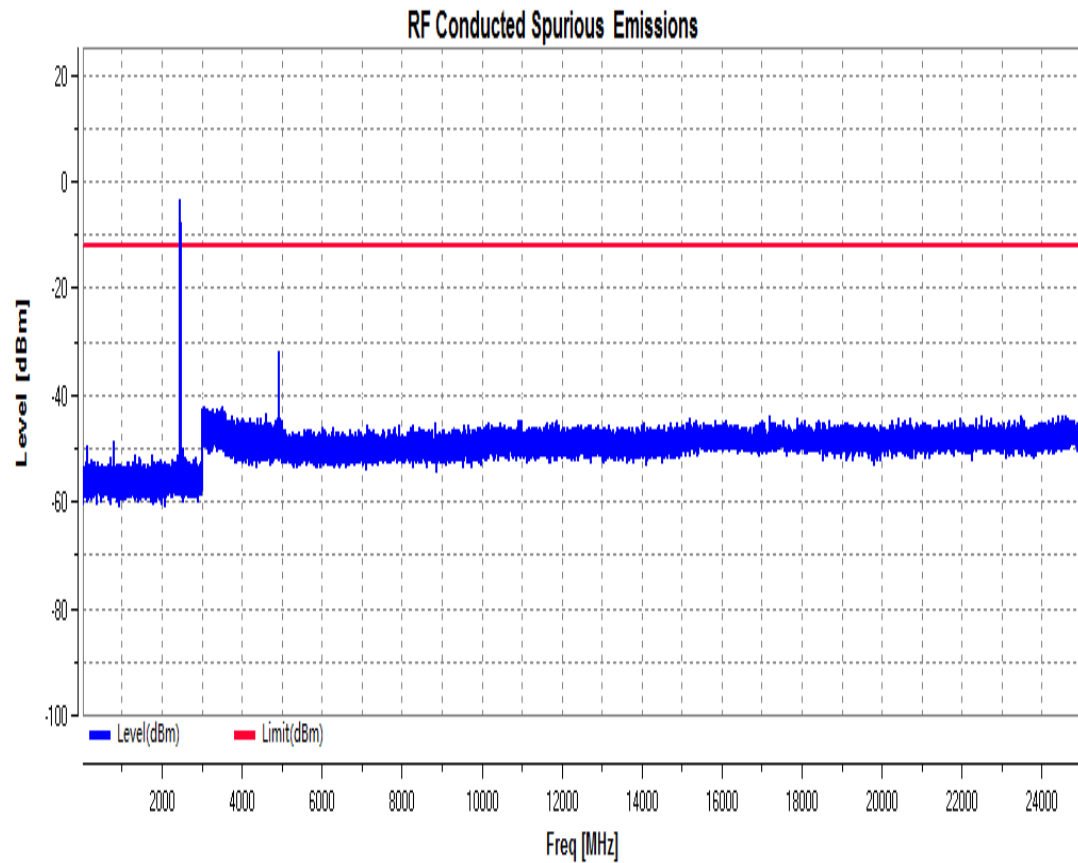
RF Conducted Spurious Emissions_11N20SISO_2462_Ant2
