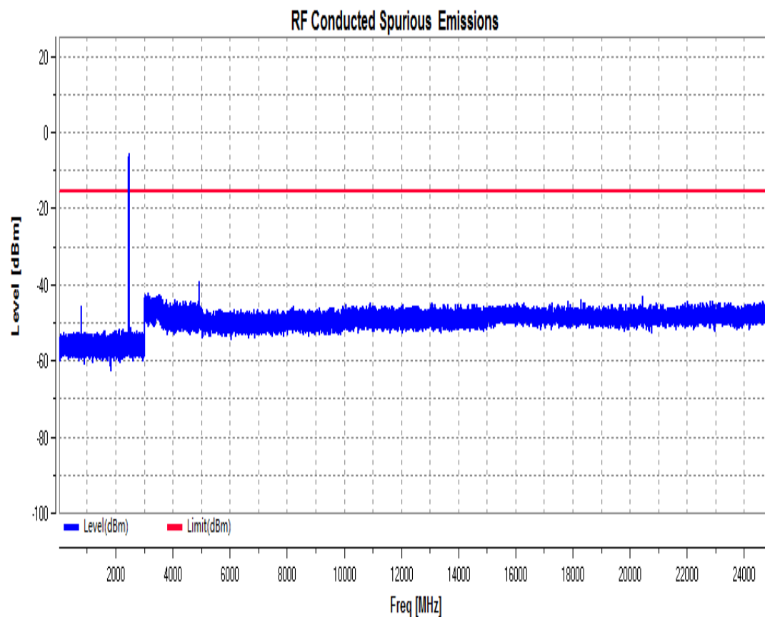
RF Conducted Spurious Emissions_11G_2462_Ant1
