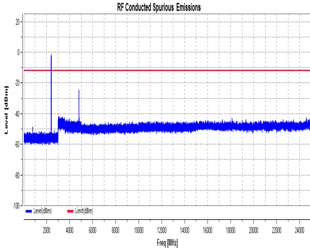
RF Conducted Spurious Emissions_11B_2412_Ant2
