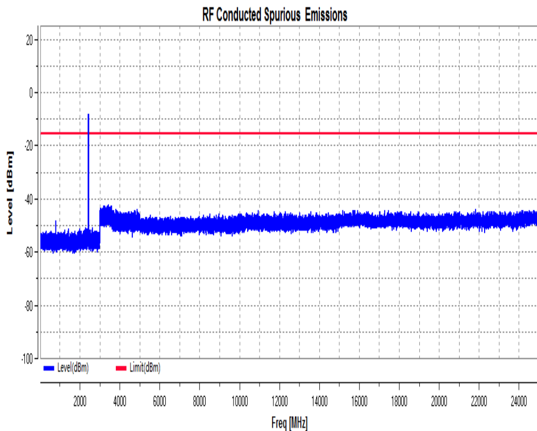
RF Conducted Spurious Emissions_11N20MIMO_2437_Ant1+2
