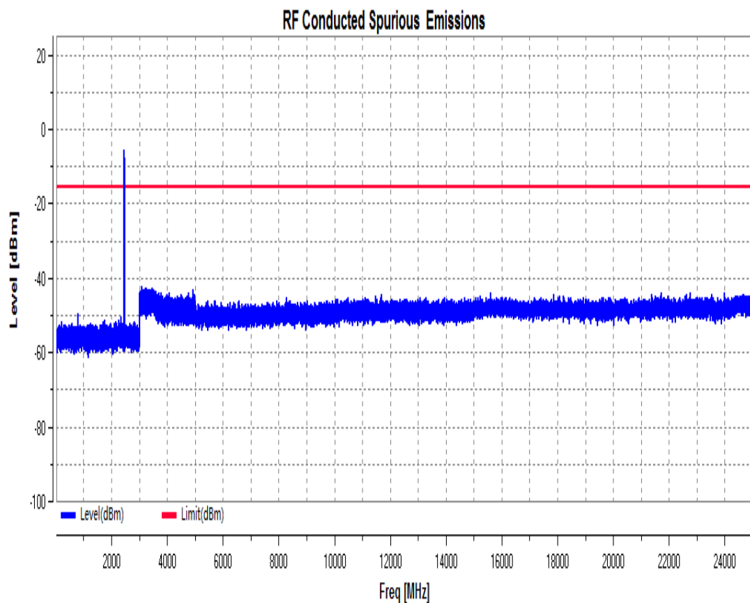
RF Conducted Spurious Emissions_11G_2462_Ant2
