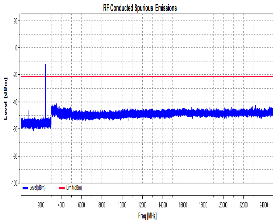
RF Conducted Spurious Emissions_11N40SISO_2452_Ant1
