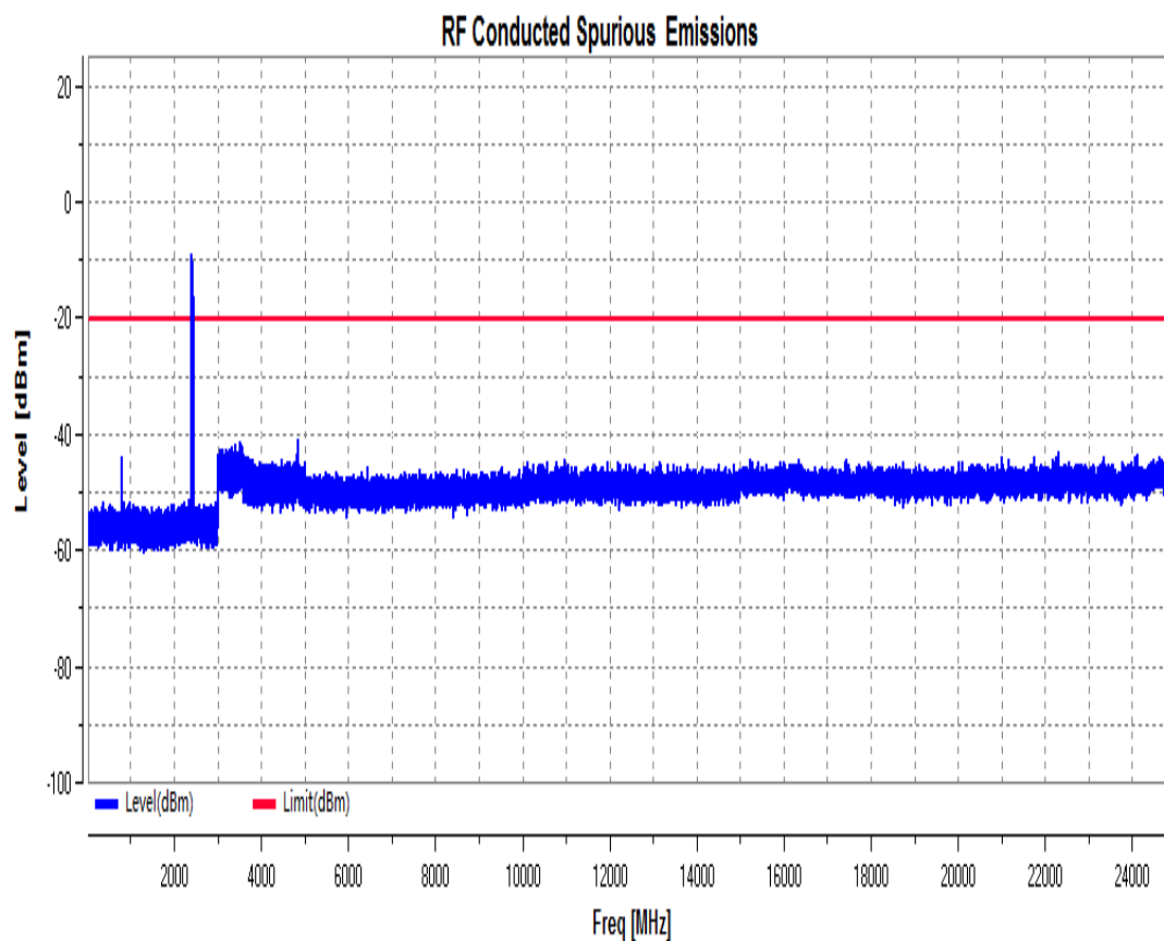
RF Conducted Spurious Emissions_11N40SISO_2422_Ant1
