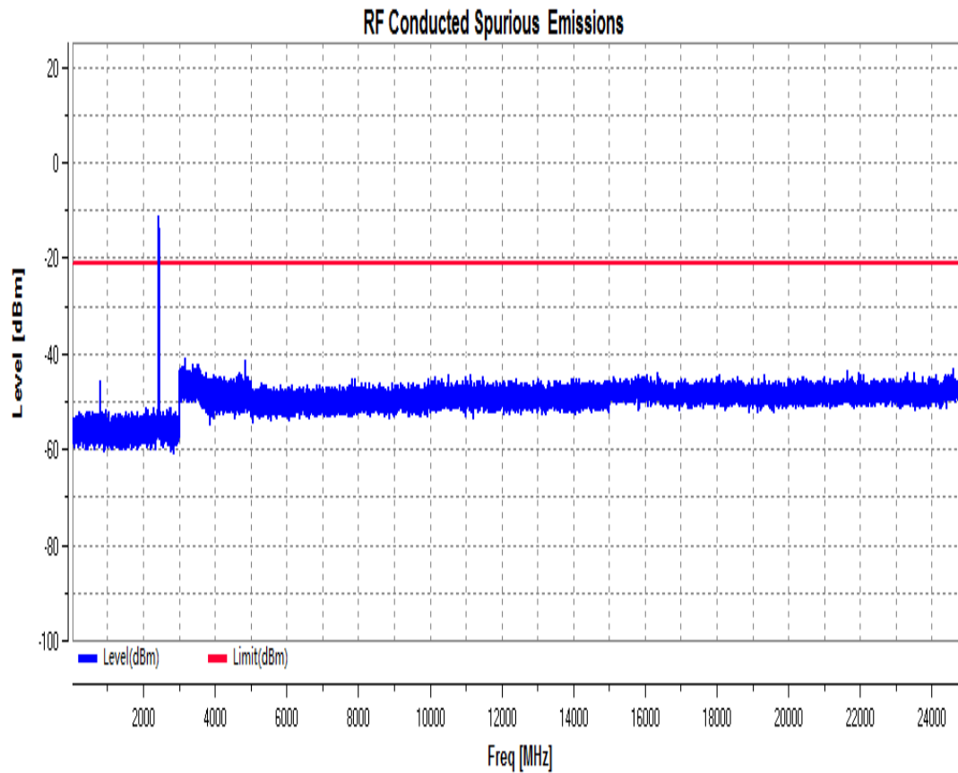
RF Conducted Spurious Emissions_11N40SISO_2437_Ant1
