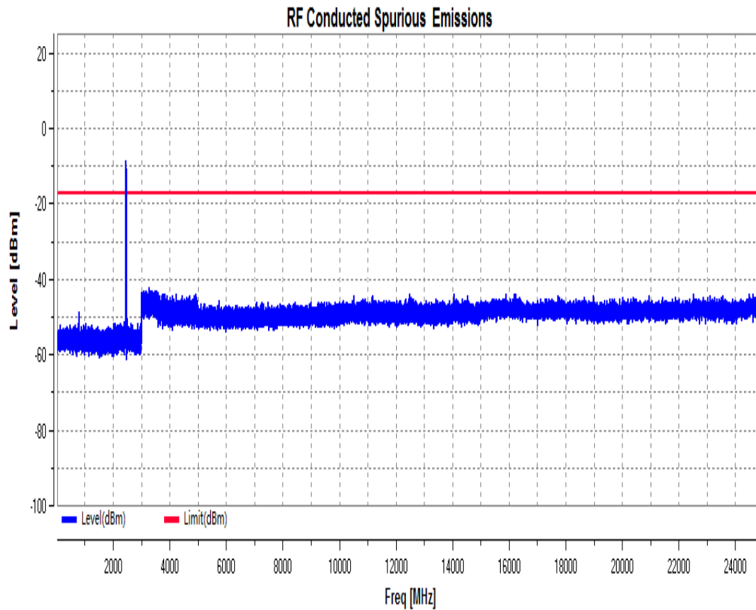
RF Conducted Spurious Emissions_11N20SISO_2462_Ant2
