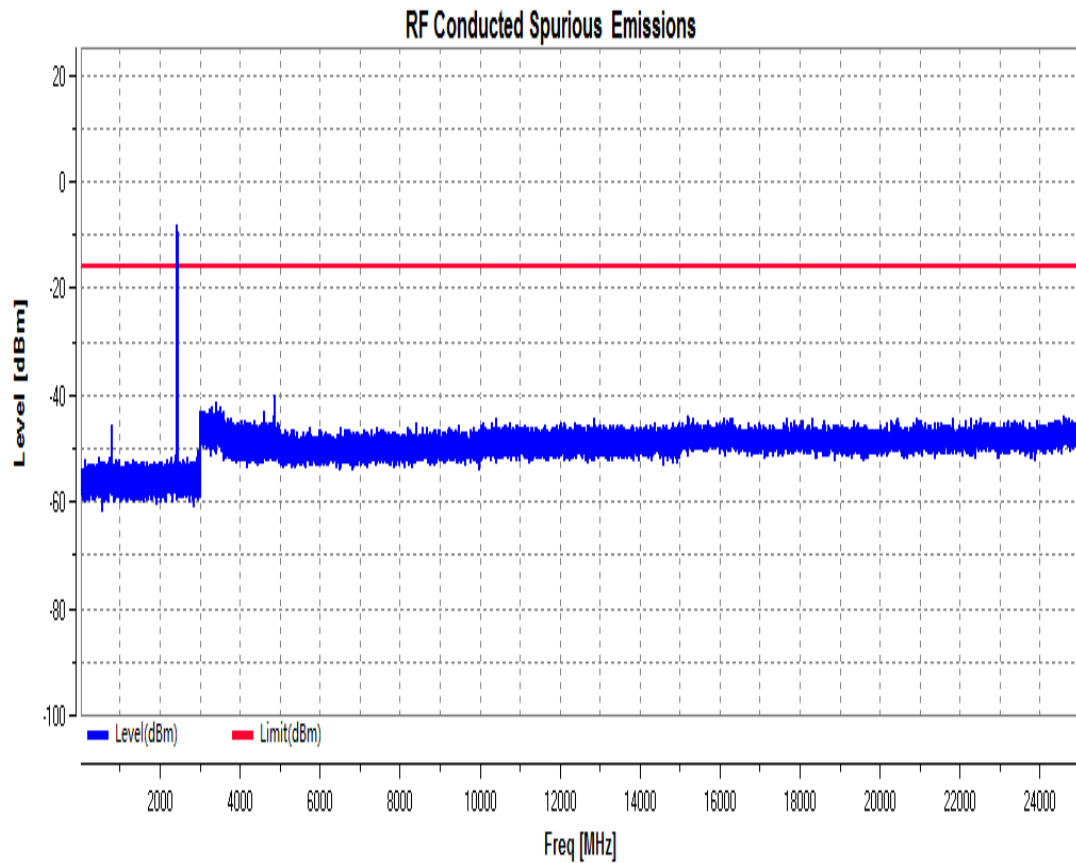
RF Conducted Spurious Emissions_11G_2437_Ant1
