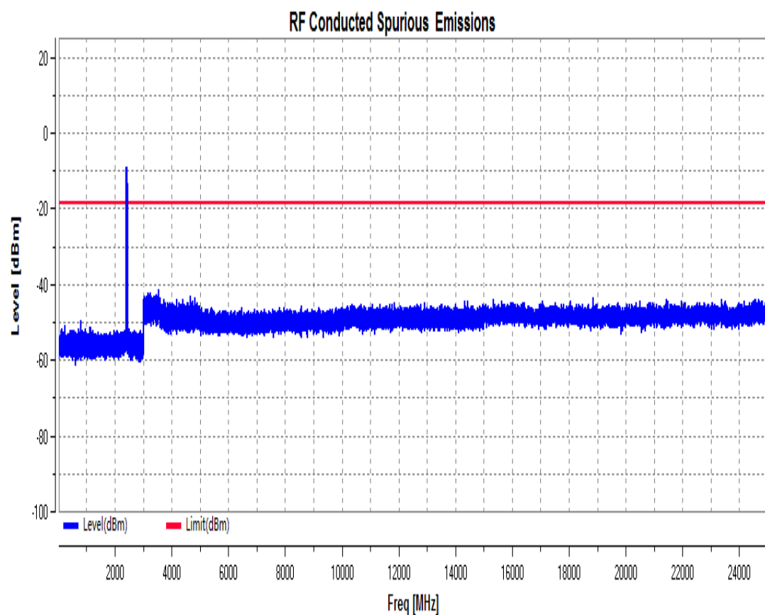
RF Conducted Spurious Emissions_11N40MIMO_2422_Ant1+2
