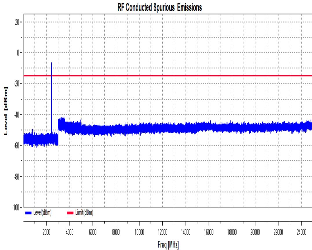
RF Conducted Spurious Emissions_11N20MIMO_2462_Ant1+2
