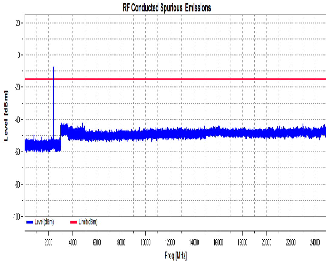
RF Conducted Spurious Emissions_11N20MIMO_2412_Ant1+2
