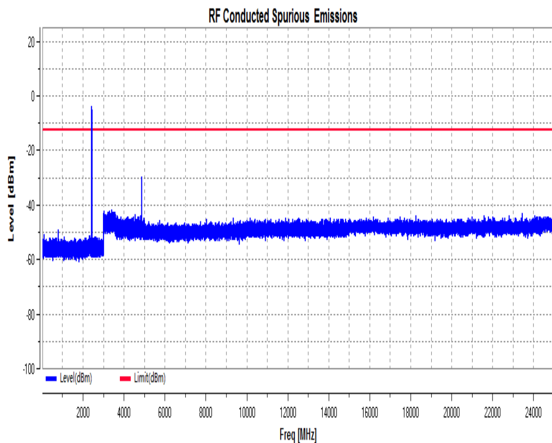
RF Conducted Spurious Emissions_11N20SISO_2437_Ant2
