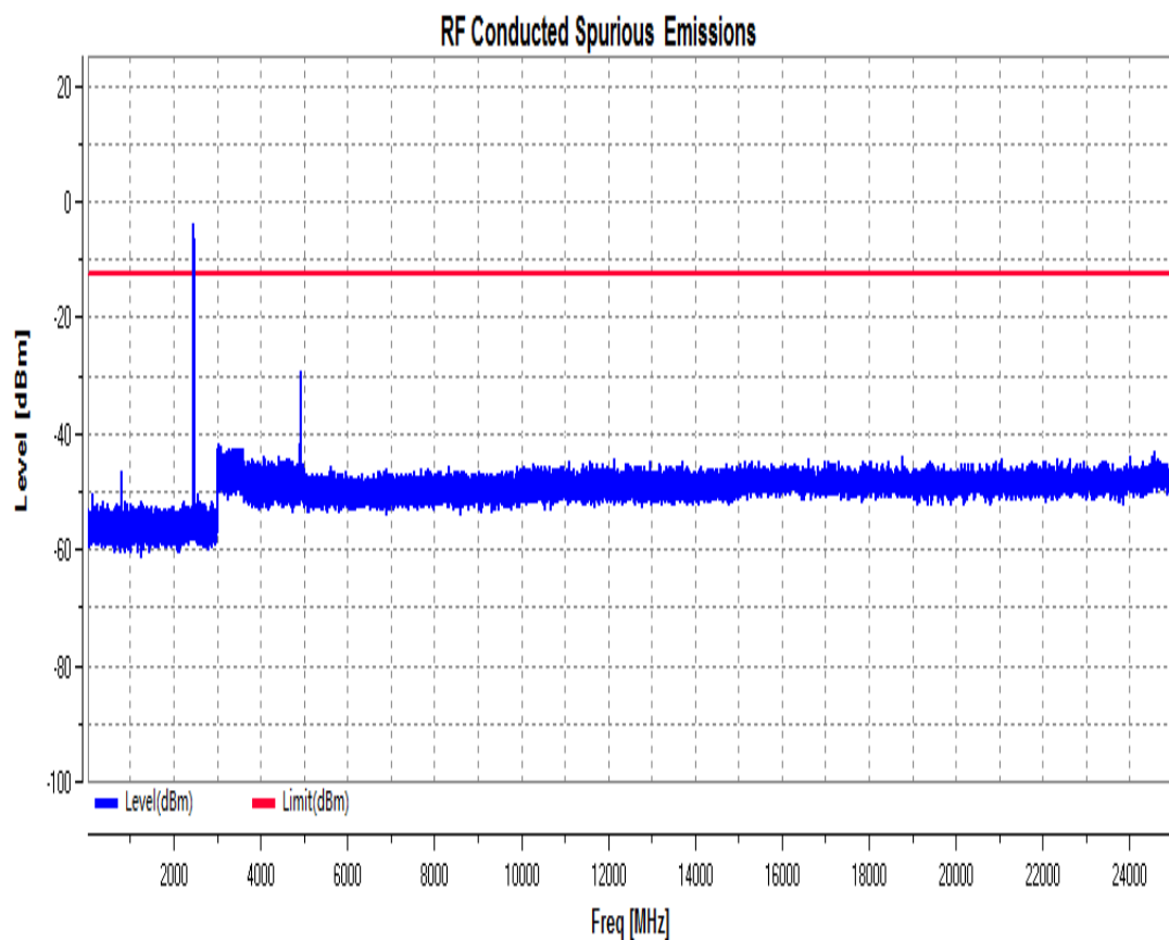
RF Conducted Spurious Emissions_11G_2412_Ant1
