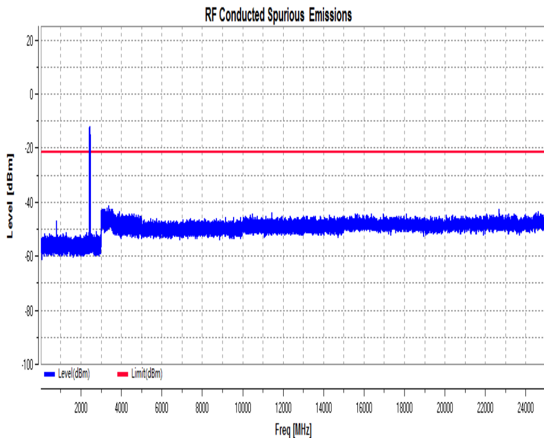
RF Conducted Spurious Emissions_11N40SISO_2452_Ant2
