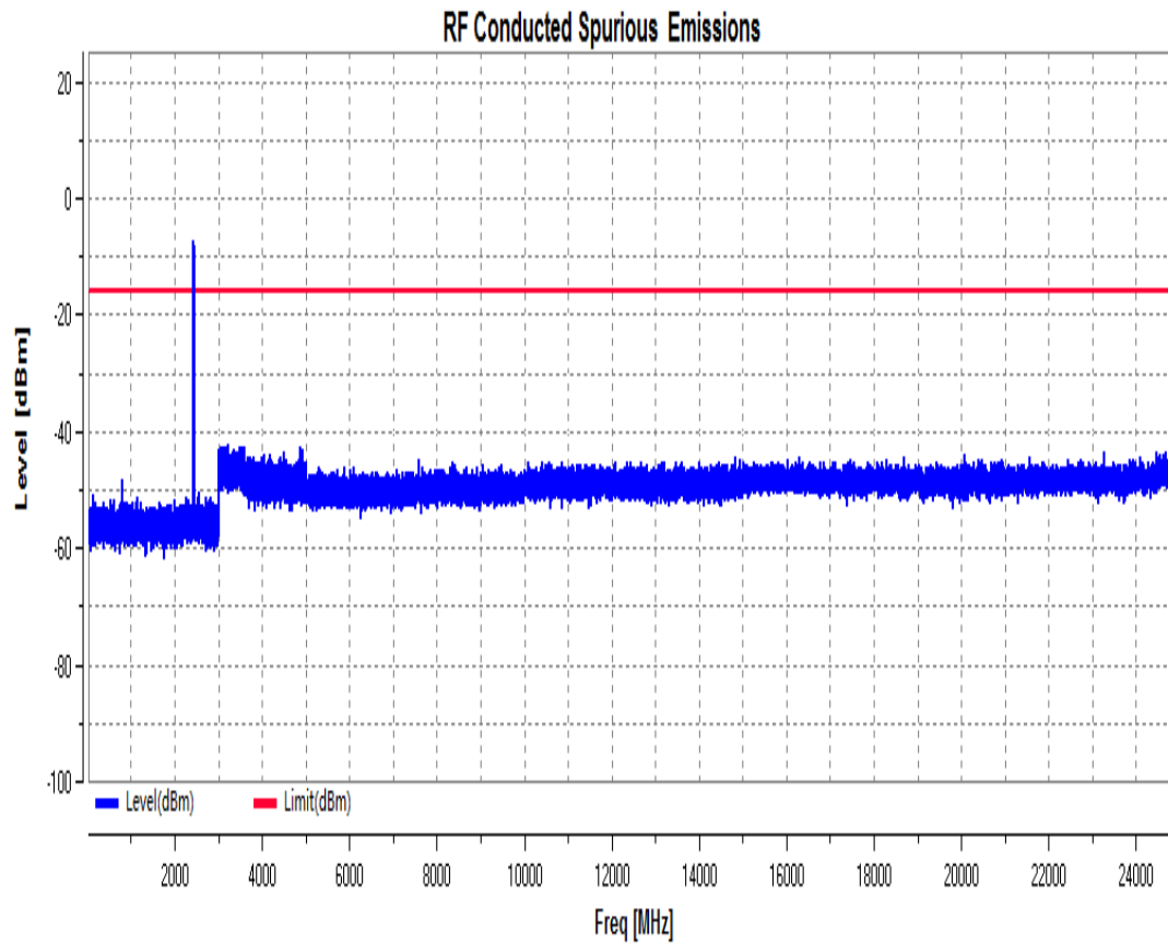
RF Conducted Spurious Emissions_11G_2437_Ant2
