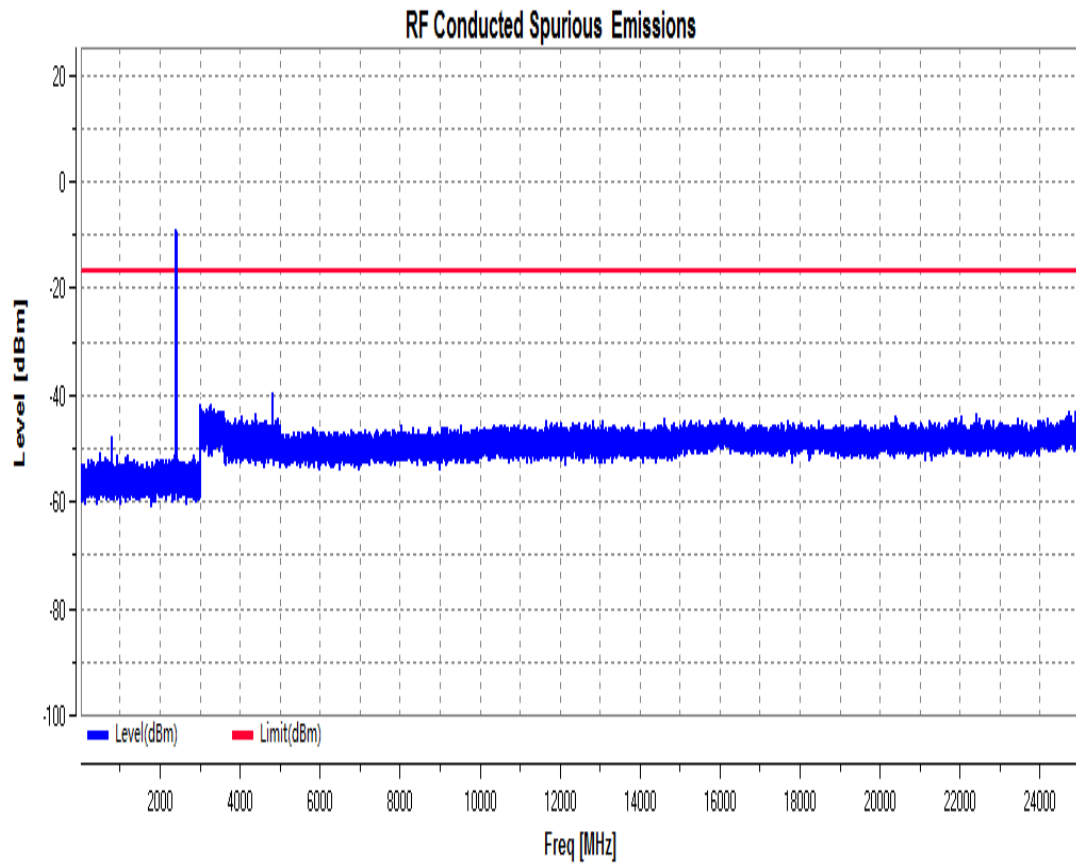
RF Conducted Spurious Emissions_11N20SISO_2412_Ant2
