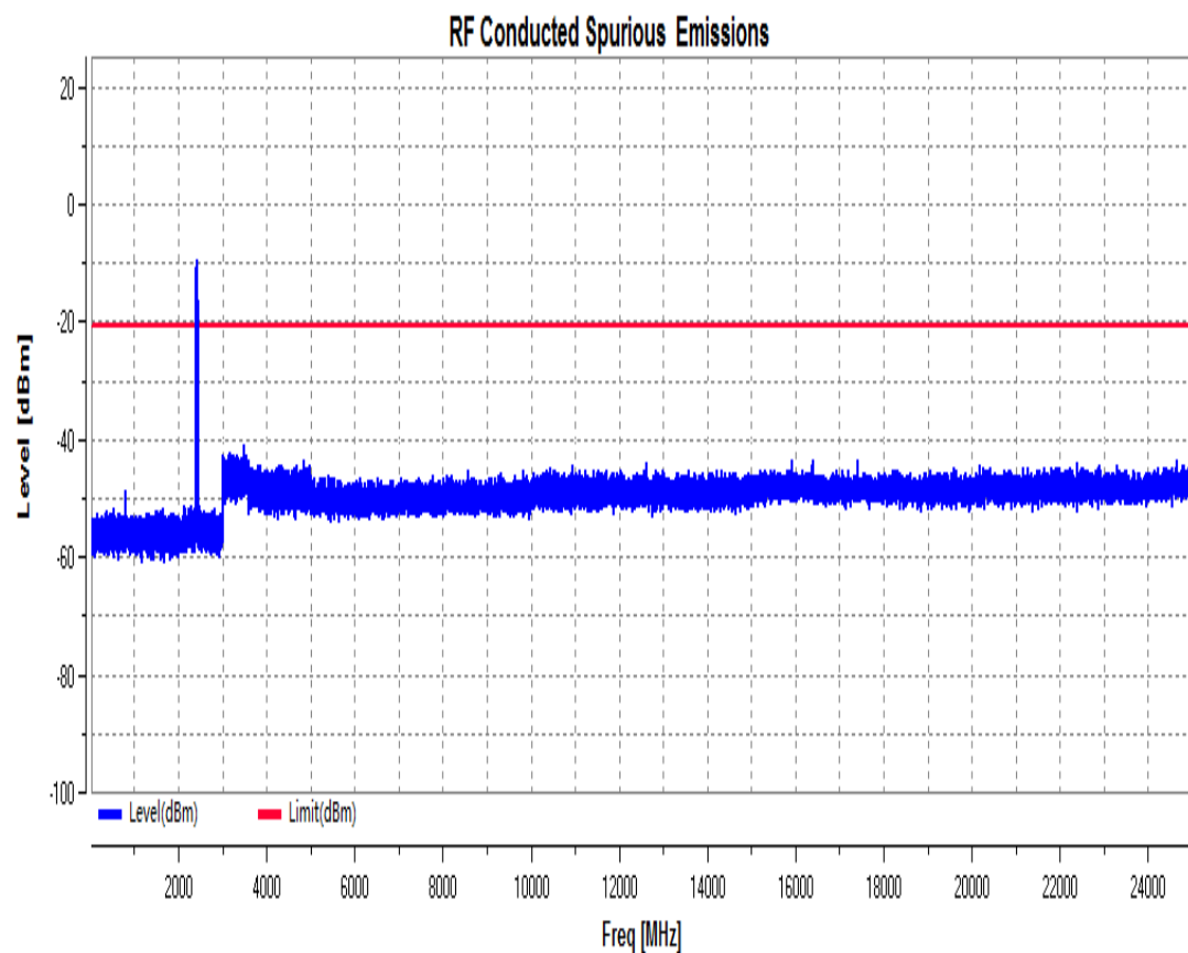
RF Conducted Spurious Emissions_11N40SISO_2422_Ant2
