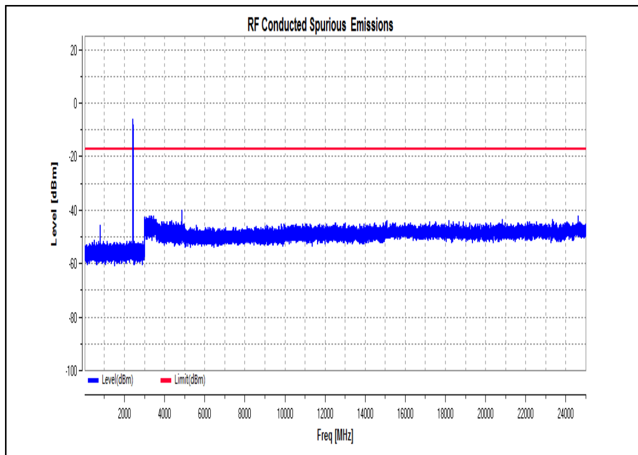
RF Conducted Spurious Emissions_11N20SISO_2437_Ant1
