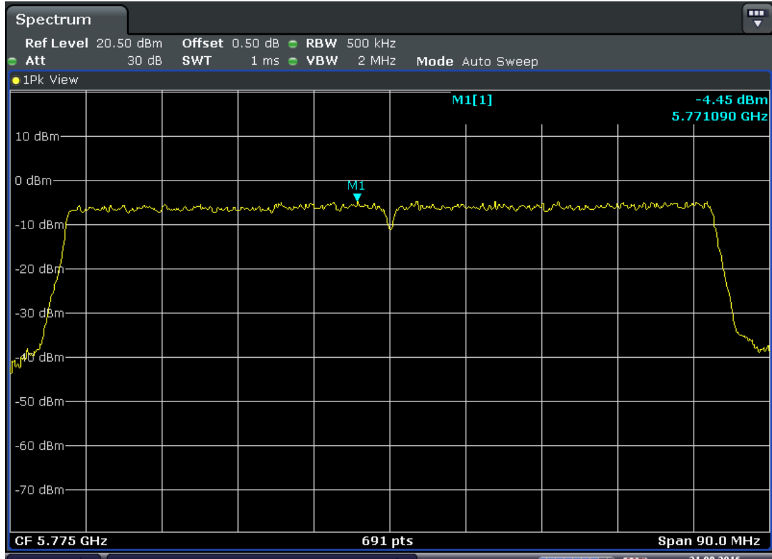
5775MHz-Ant2
