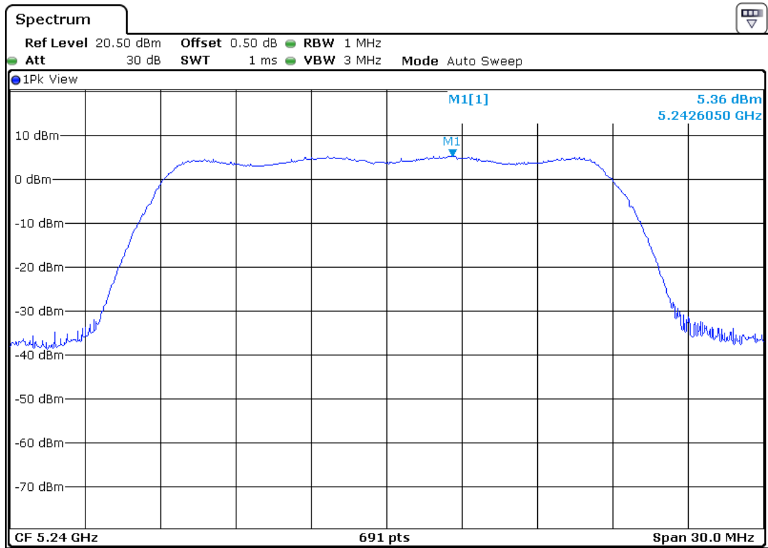
5240MHz-Ant2
