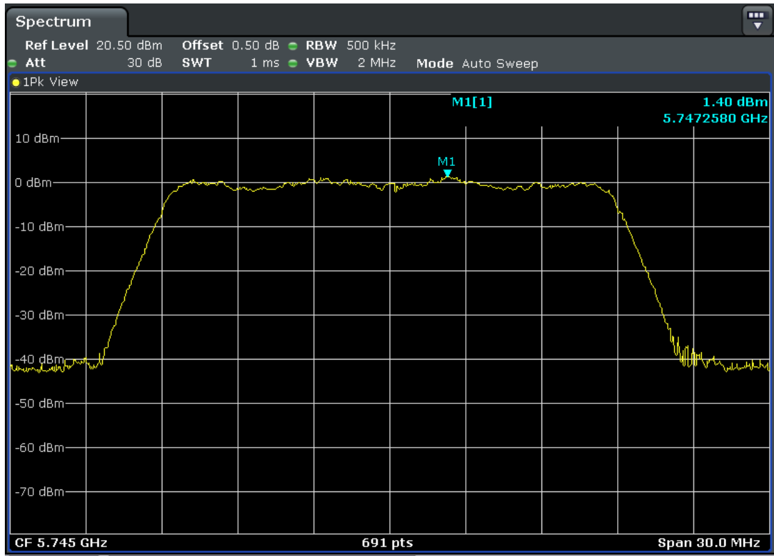
5745MHz-Ant2
