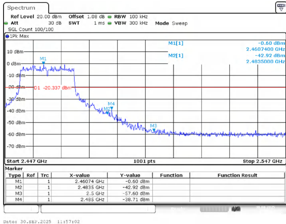
Band Edge NVNT ax20 2462MHz Ant1 Emission
