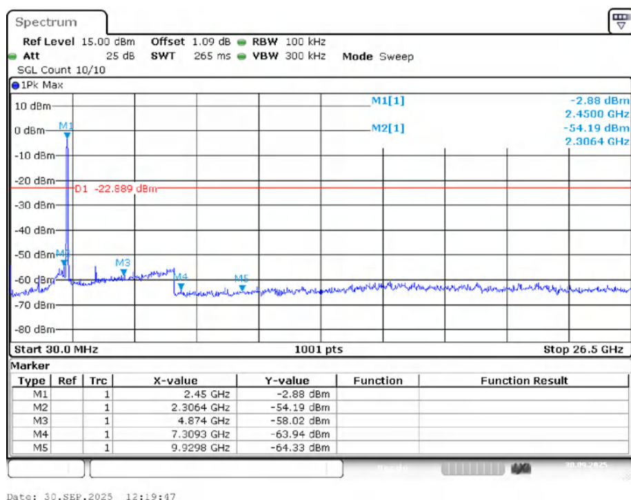
Tx. Spurious NVNT ax40 2452MHz Ant1 Emission
