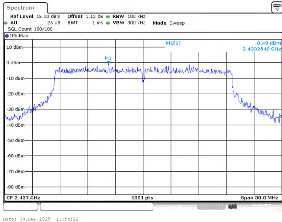
Tx. Spurious NVNT ax20 2437MHz Ant1 Ref
