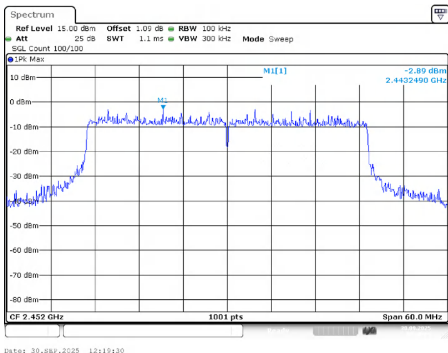
Tx. Spurious NVNT ax40 2452MHz Ant1 Ref
