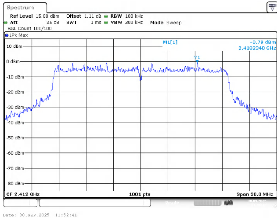
Tx. Spurious NVNT ax20 2412MHz Ant1 Ref
