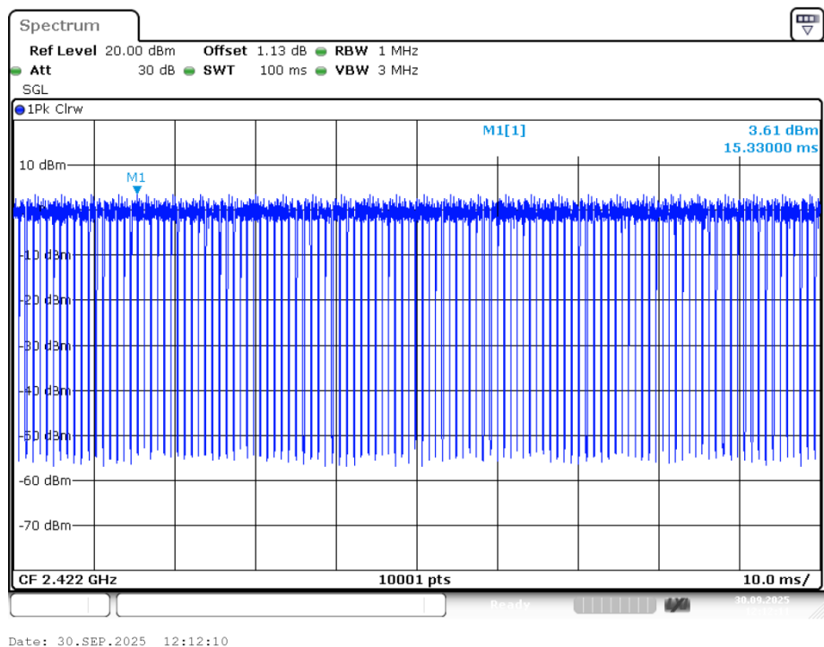
Duty Cycle NVNT ax40 2422MHz Ant1
