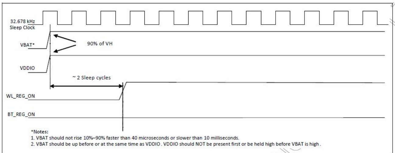
WLAN=ON, Bluetooth=OFF
