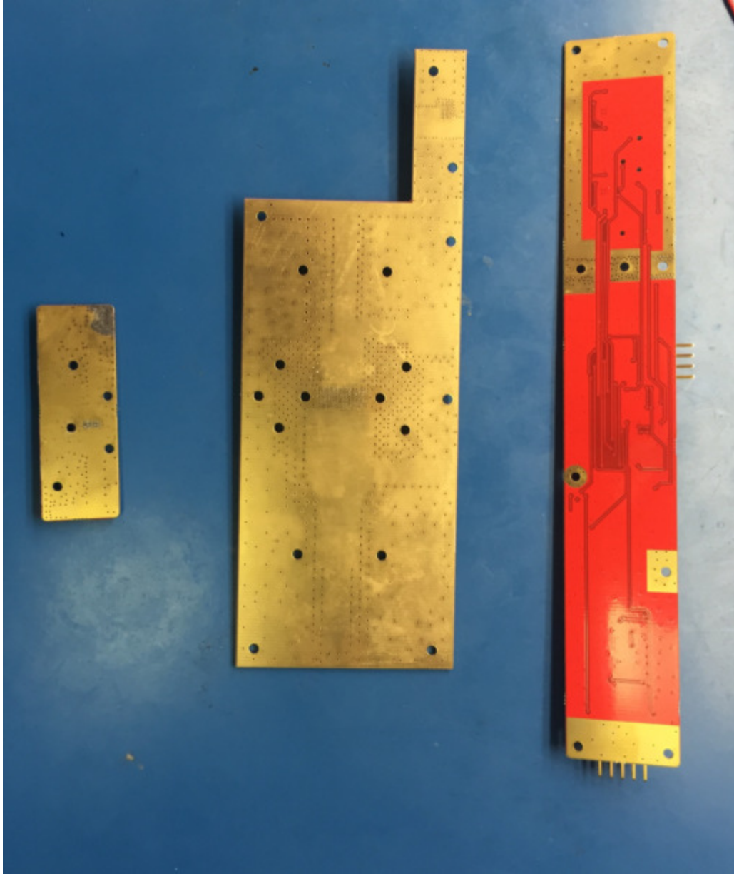
PCB Back Side – PA Driver, PA and PA Controller
