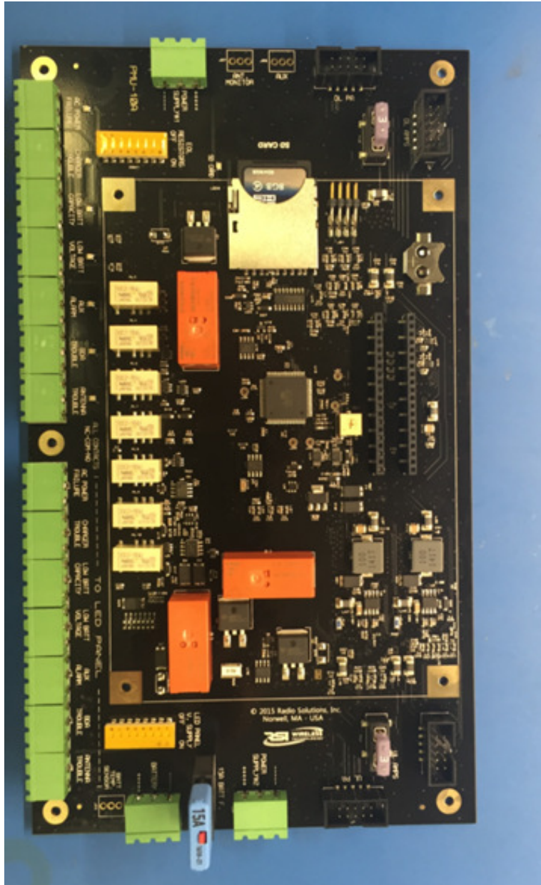
Power Management and Alarm Interface*
