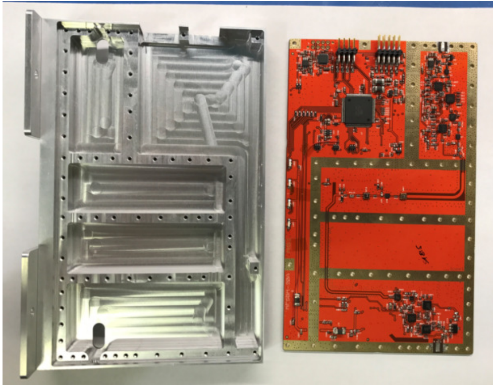
RF Module Component Side
