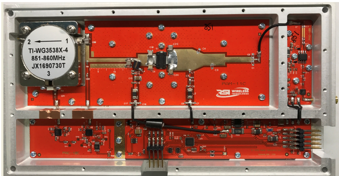
Power Amplifier Module with PA Controller and PA Driver
