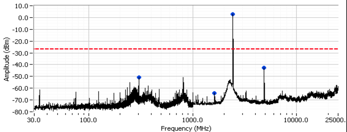
802.11b Ch #6 (Power setting: 18)
