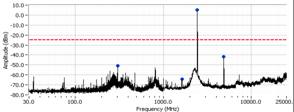
802.11g Ch #6 (Power setting: 21)
