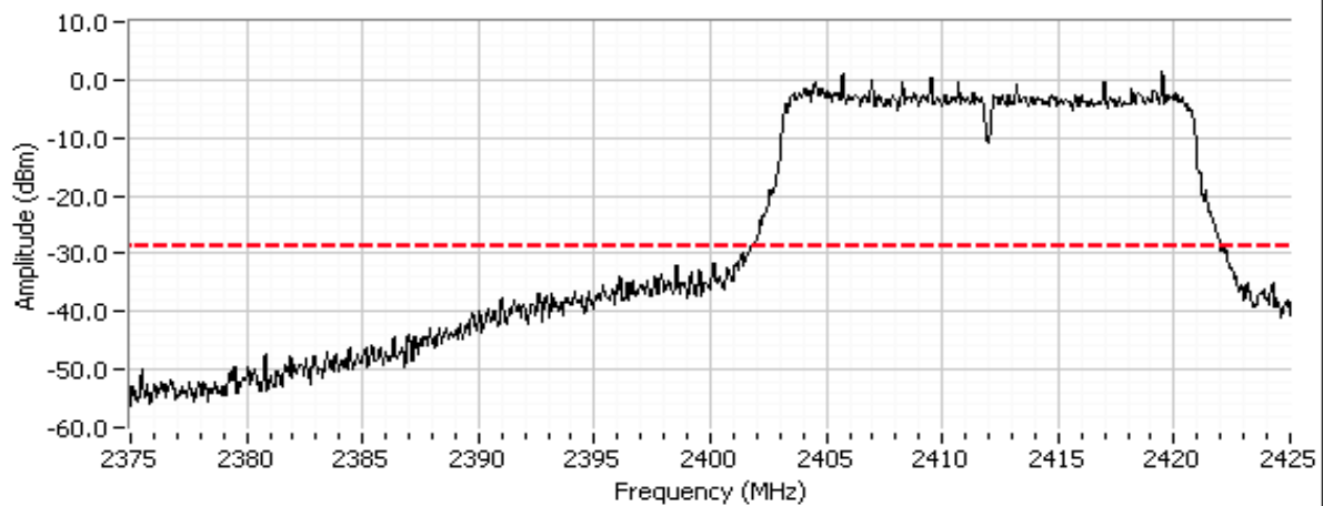
802.11n20 Ch #1 (Power setting: 13)
