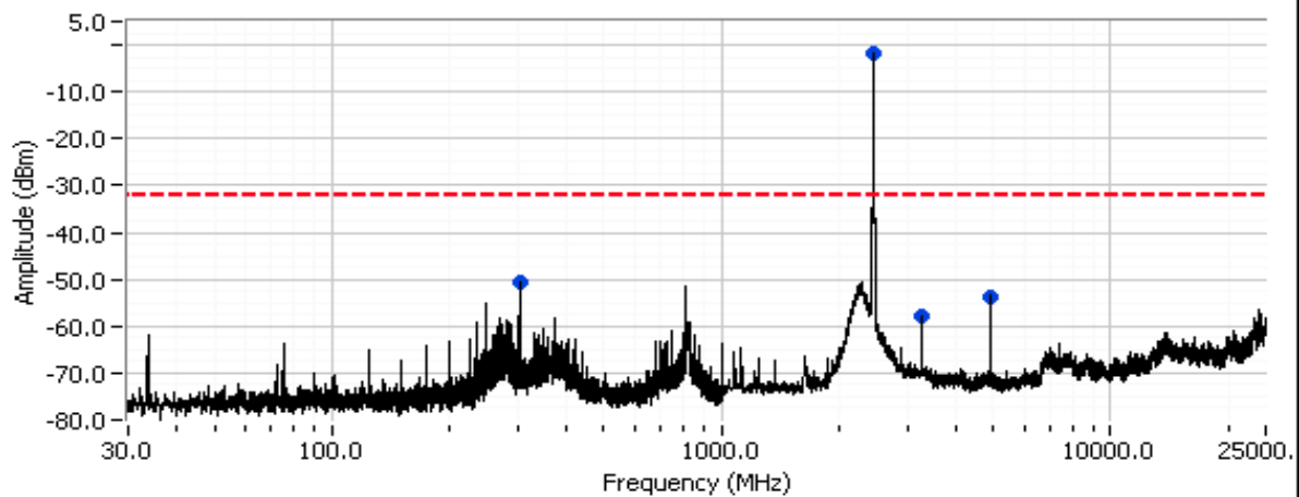
802.11n20 Ch #11 (Power setting: 16)
