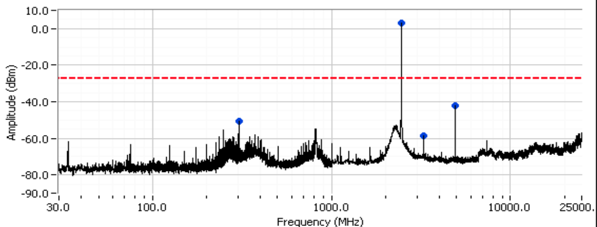
802.11b Ch #11 (Power setting: 18)
