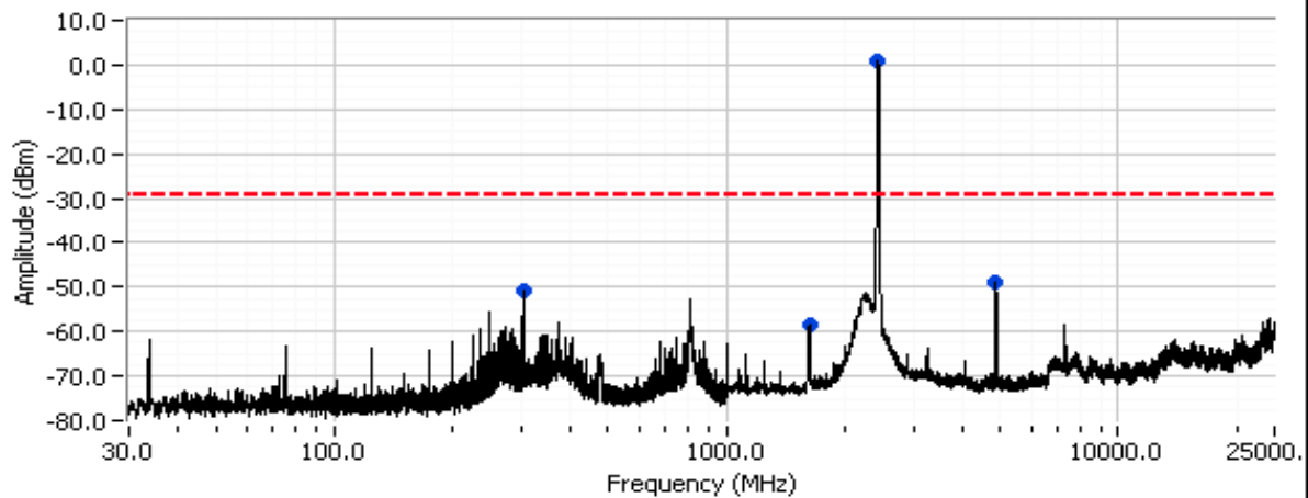
802.11n20 Ch #6 (Power setting: 21)
