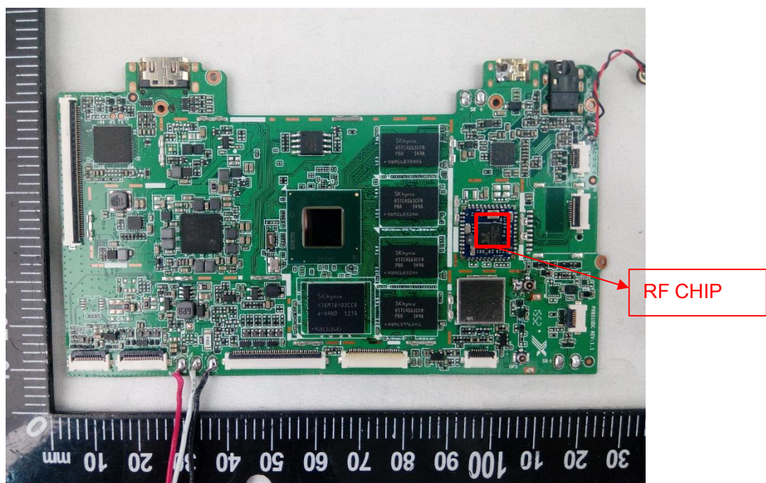
MAIN BOARD FRONT VIEW 2
