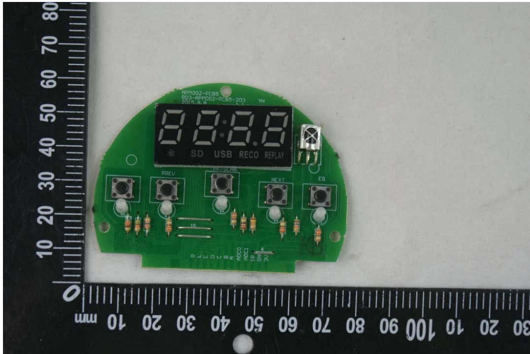
MAIN BOARD 6 FRONT VIEW
