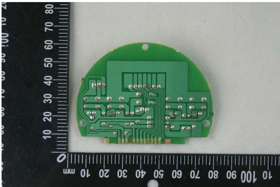
MAIN BOARD 6 BACK VIEW
