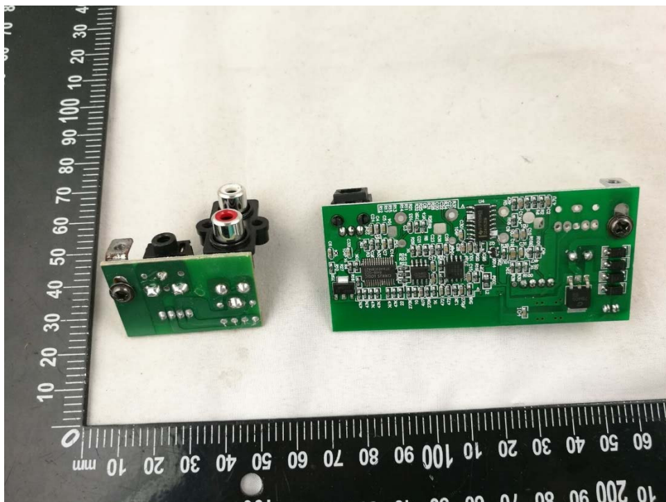
MAIN BOARD 5 FRONT VIEW
