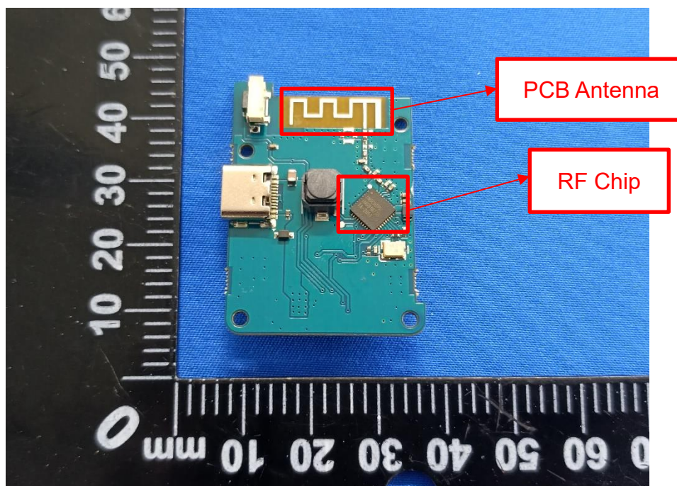
MAIN BOARD TOP VIEW (WITH SHIELDING)
