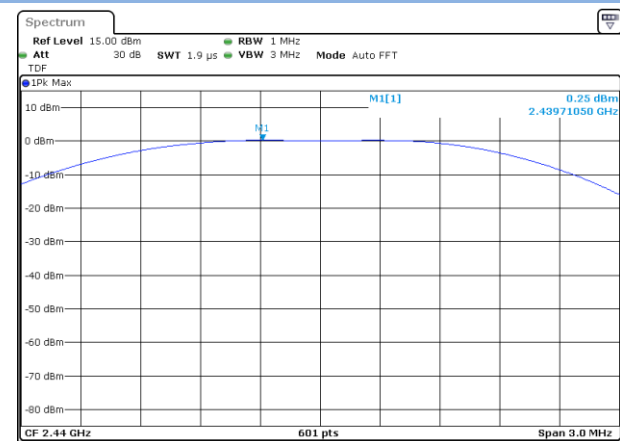
GFSK(BLE) MIDDLE CHANNEL
