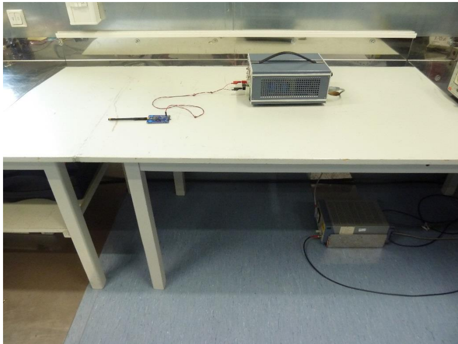
Photo 4 (Conducted AC emissions):
