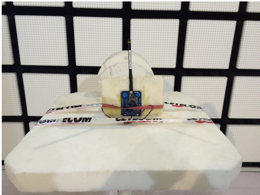
Photo 2 (RSE setup – 9kHz to 30MHz & 1GHz to 10GHz):
