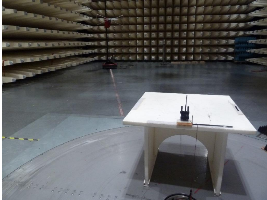
Photo 1 (RSE setup – 30MHz to 1 GHz):
