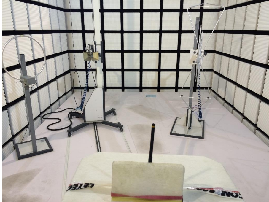
Photo 3 (RSE setup – 9kHz to 30MHz & 1GHz to 10GHz):
