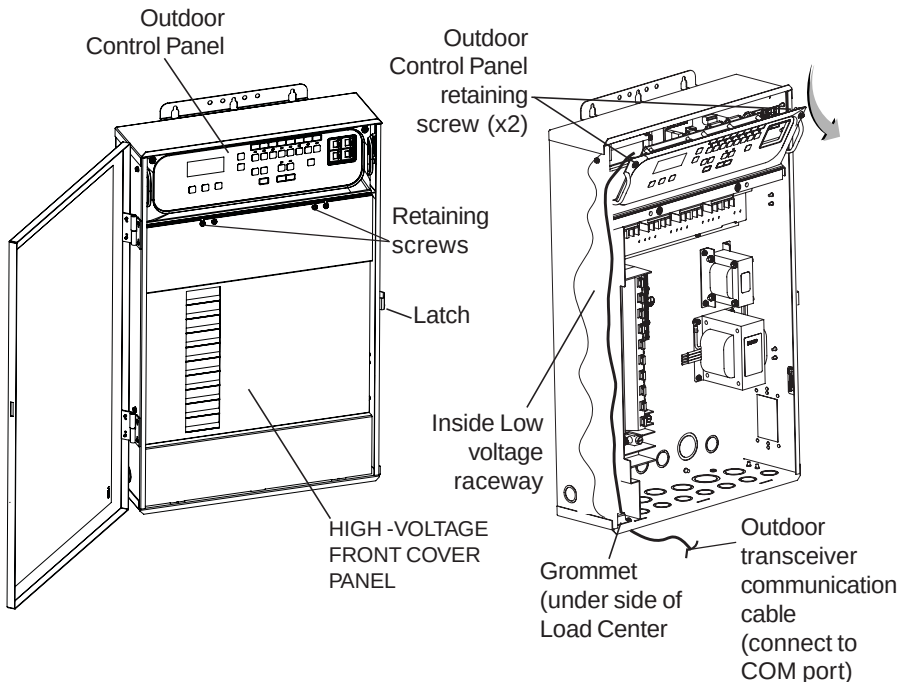
IntelliTouch® or EasyTouch® Control System Load Center
