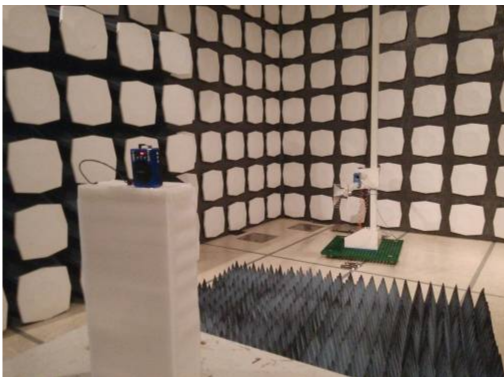
Re ( Above1GHz )
