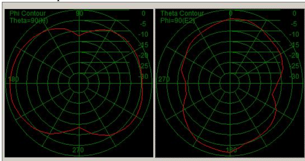
Radiation patterns:2D
