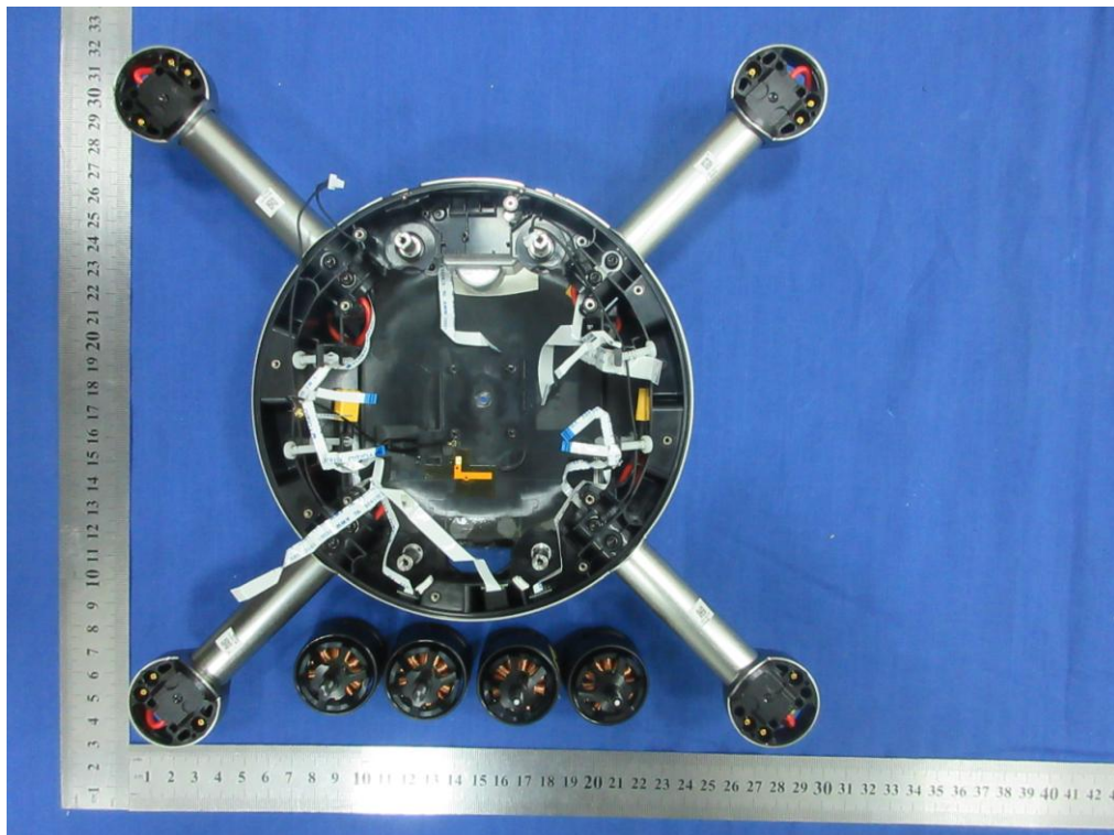
(32) EUT Photo
