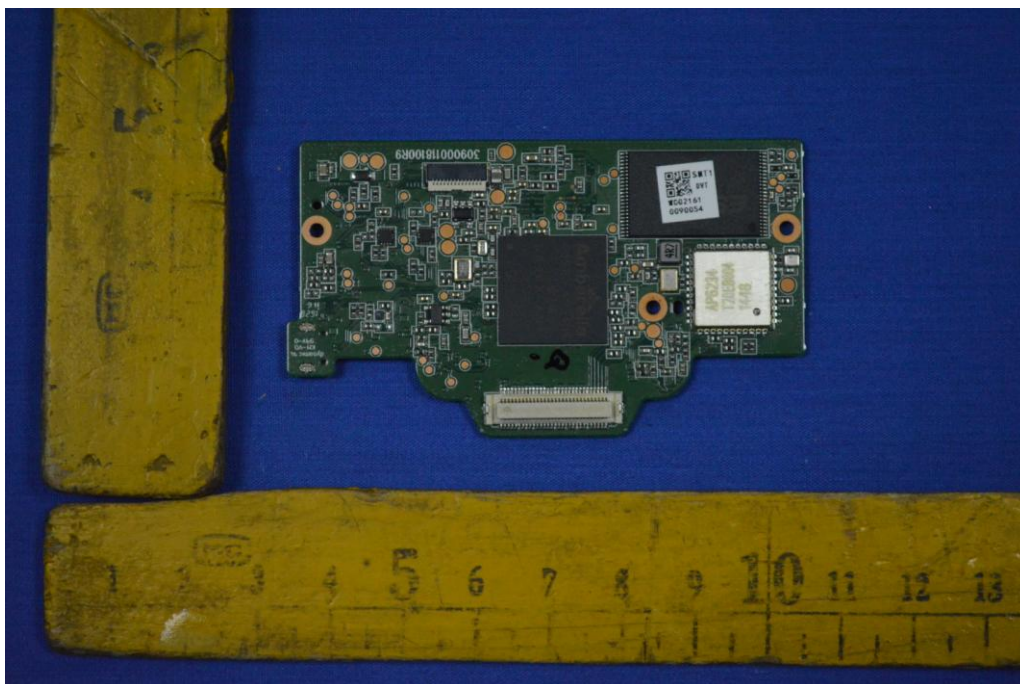
(28) EUT Photo
