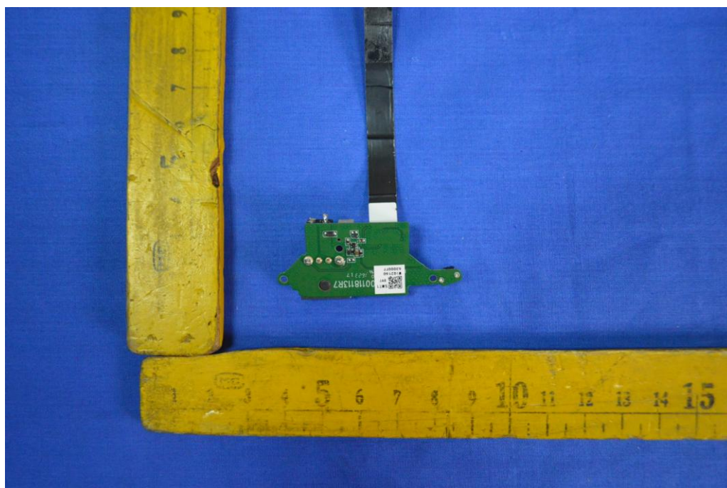
(25) EUT Photo
