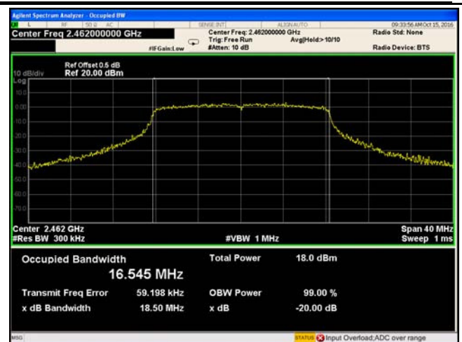
802.11g 20dB Bandwidth – CH11 2462
