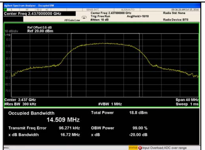
802.11b 20dB Bandwidth – CH6 2437
