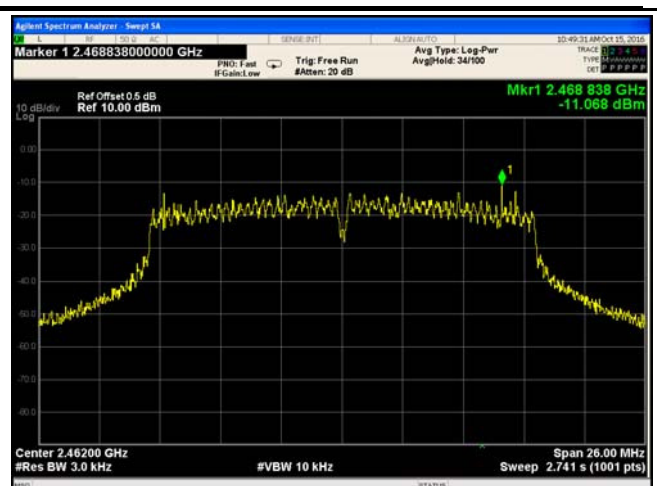
PSD - CH11 2462 – 802.11g
