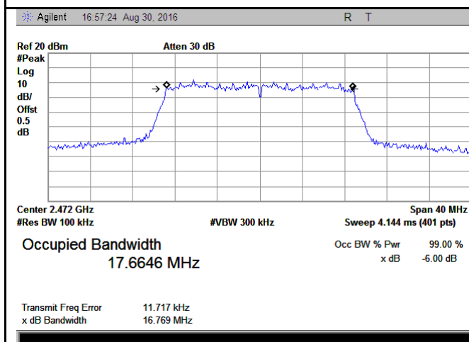
802.11n20 6dB Bandwidth – CH13 2472
