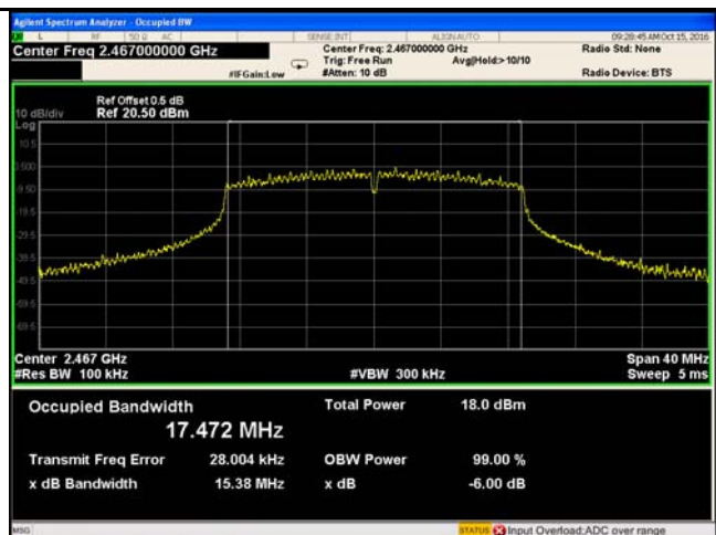
802.11n20 6dB Bandwidth – CH12 2467
