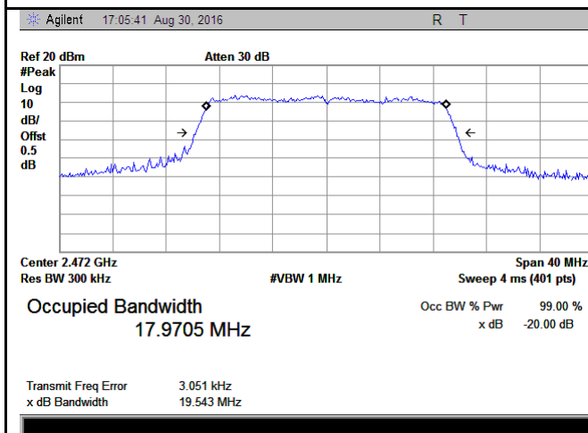
802.11n20 20dB Bandwidth – CH13 2472
