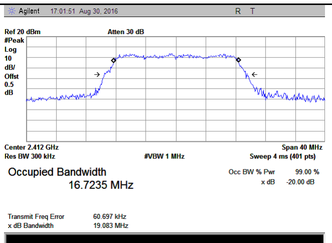
802.11g 20dB Bandwidth – CH1 2412
