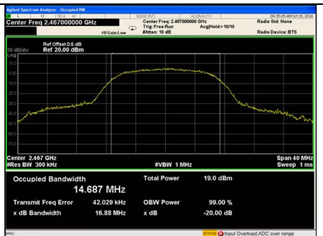
802.11b 20dB Bandwidth – CH12 2467
