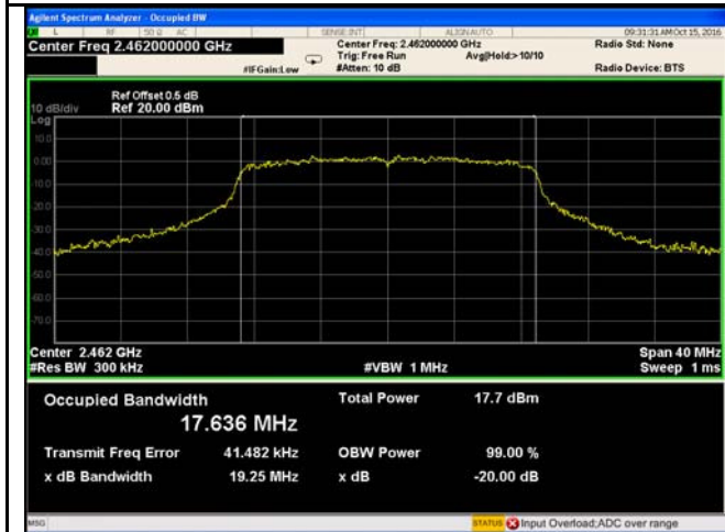
802.11n20 20dB Bandwidth – CH11 2462
