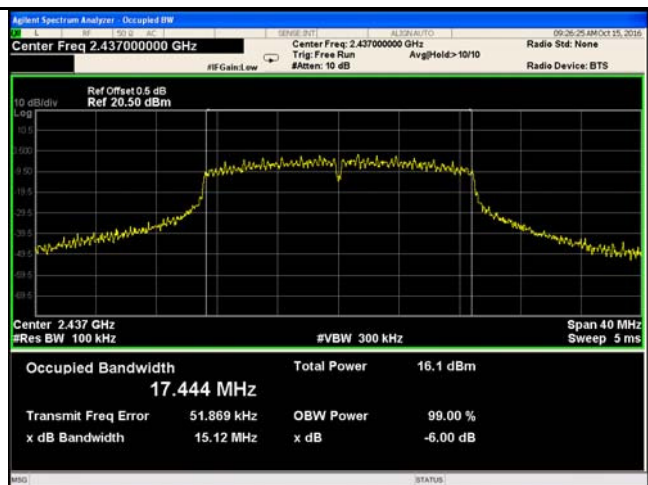
802.11n20 6dB Bandwidth – CH6 2437
