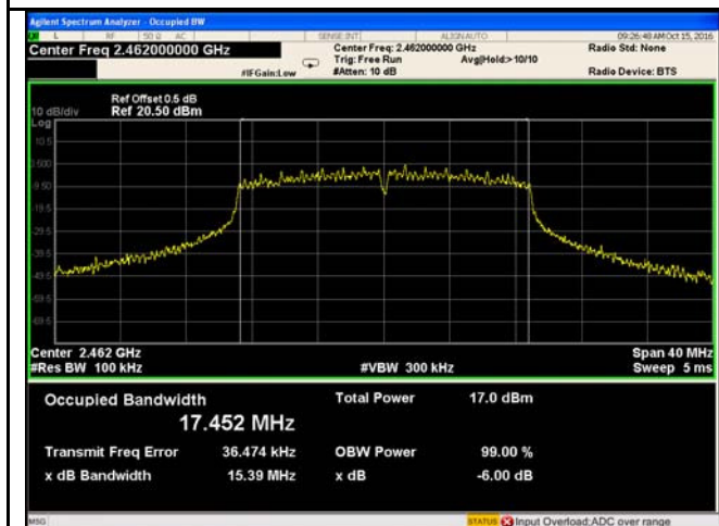
802.11n20 6dB Bandwidth – CH11 2462
