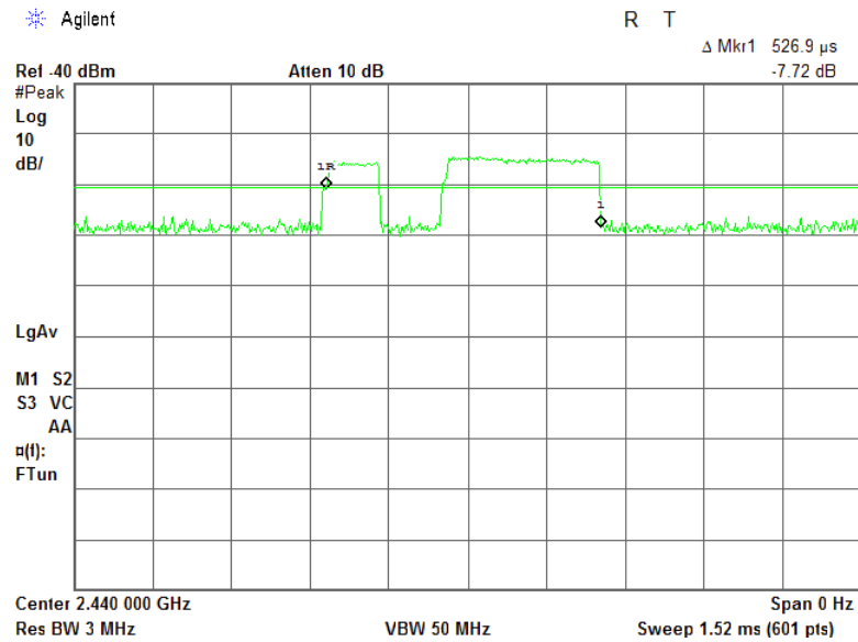
Plot 7.3.24 Transmission pulse duration
