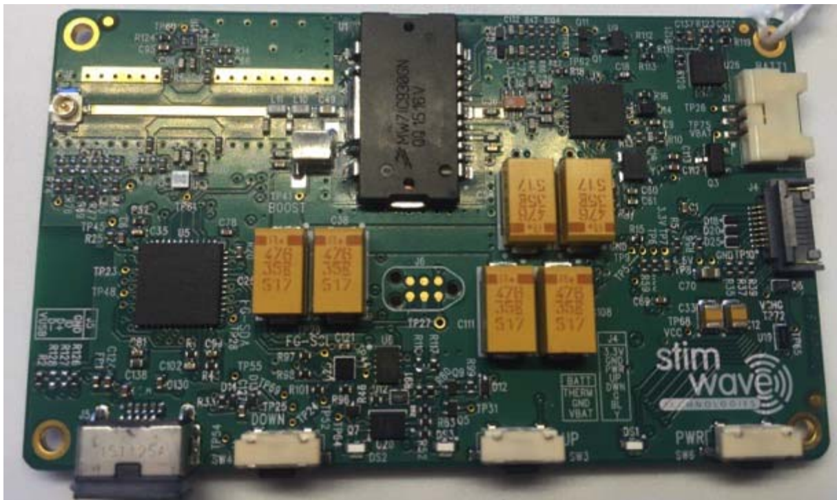
Figure 2. Top Side of the LBRD-2 Circuit board
