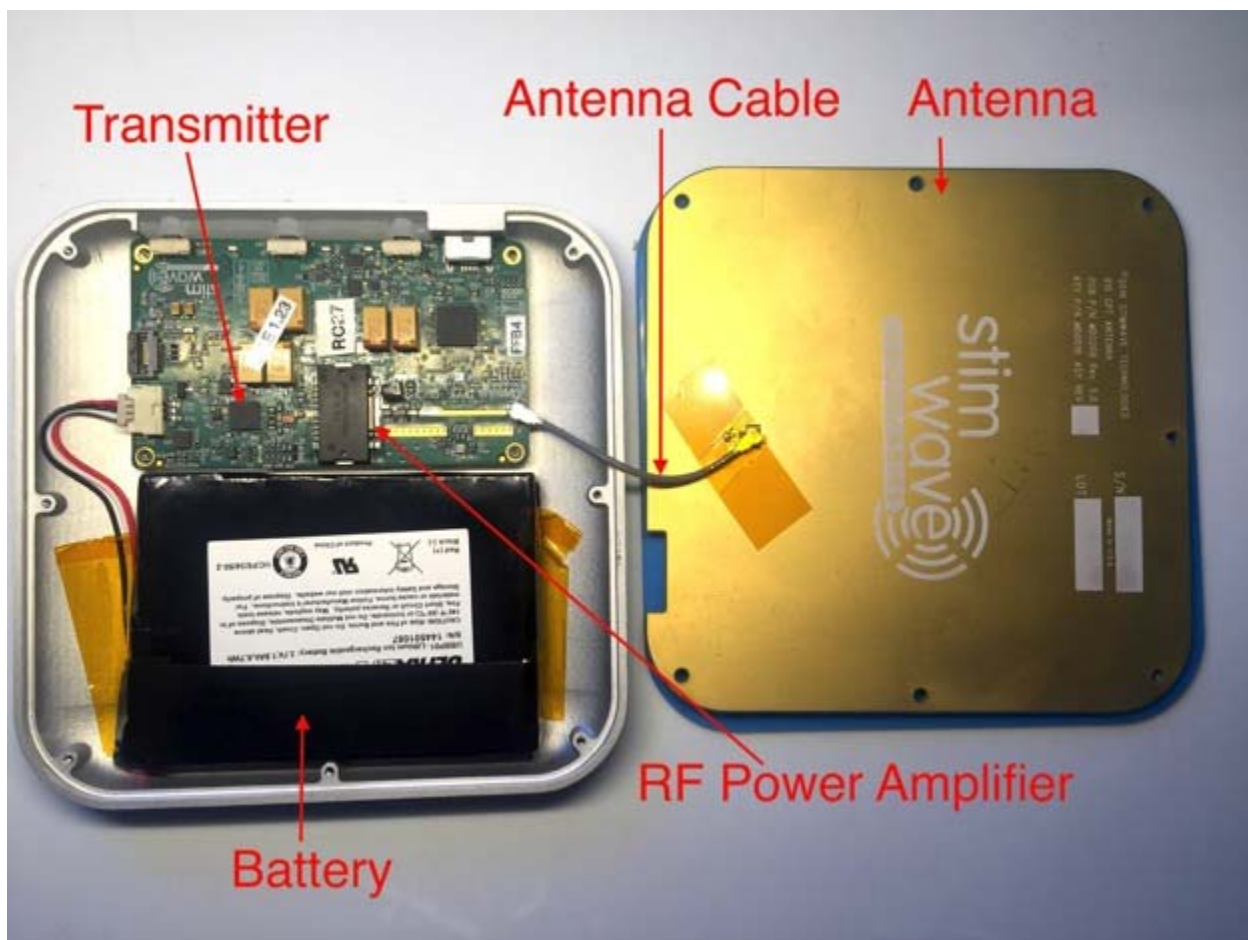
Figure 1. Overhead view of the Internals of the LBRD-2
