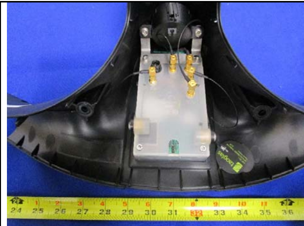
PCB View with Cover
