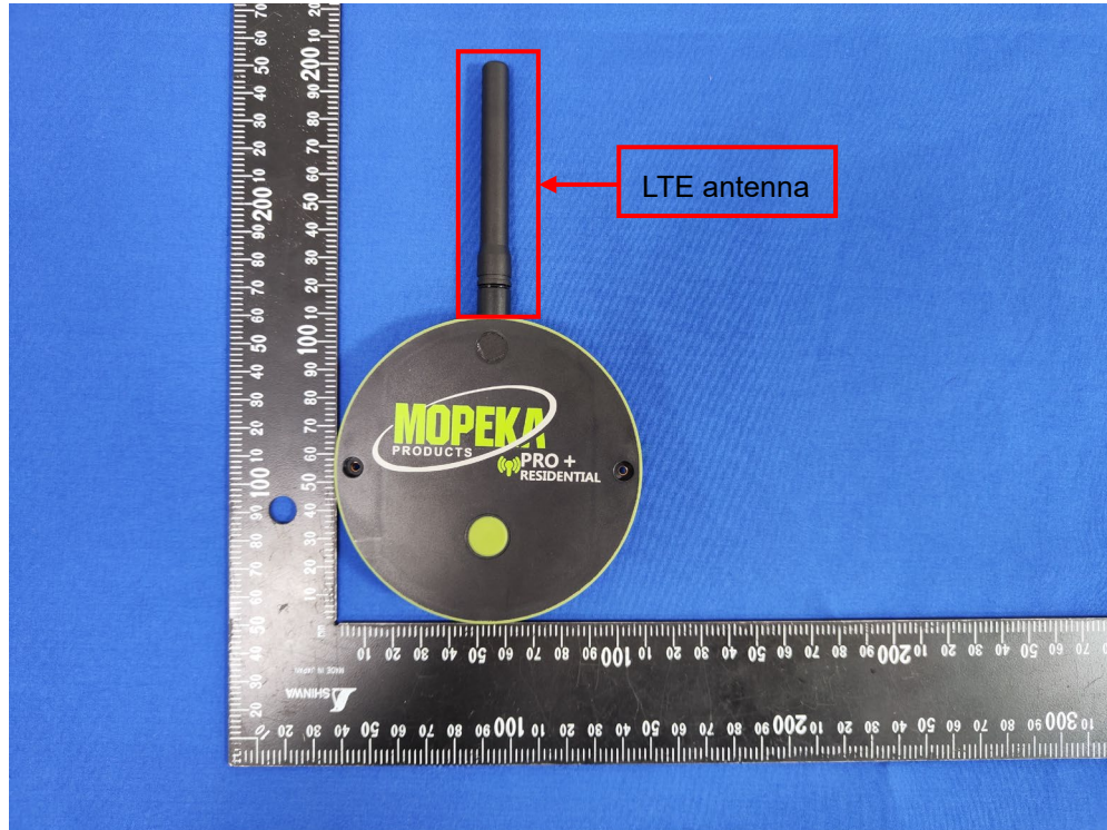
(1) EUT Photo (Top View)
