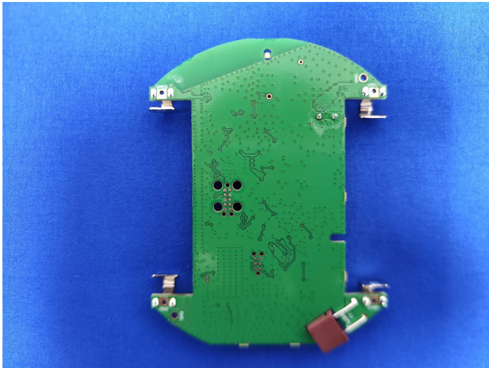
(12) EUT Photo(Antenna for BLE)
