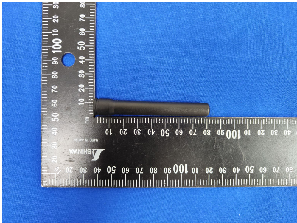
(13) EUT Photo(Antenna for LTE)
