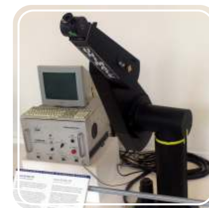
A Unimate robotic arm
