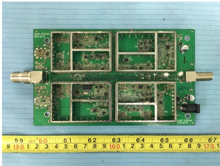
EUT – Main Board Top Shileding off View
