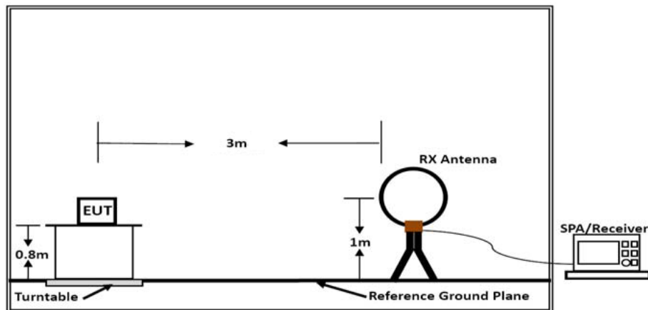
Below 30MHz
