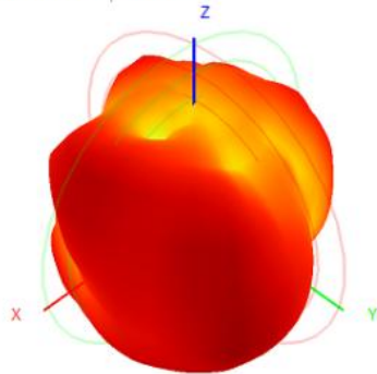
2450.0MHz H+V, Eff: 42.4%
