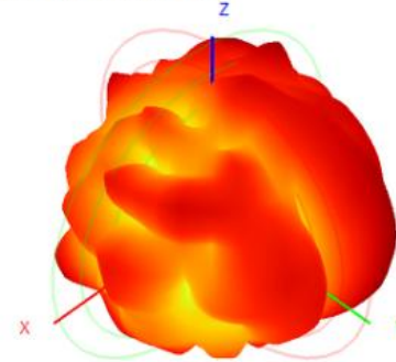
5850.0MHz H+V, Eff: 36.4%
