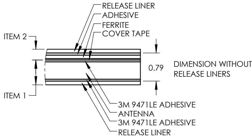
DETAIL A SCALE 16 : 1
