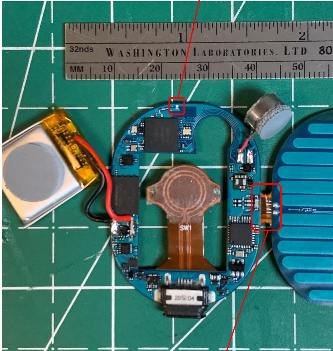
NFC Traces to 13.56MHz Antenna
