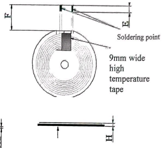
Figure 3: Coil and Magnetic Sheet Combination
