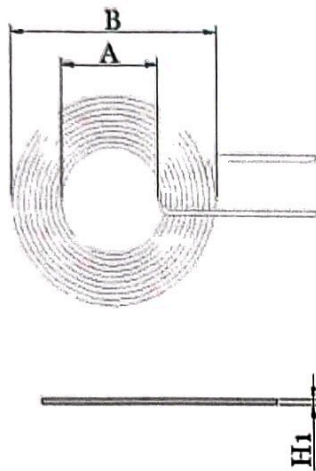
Figure 1: Coil
