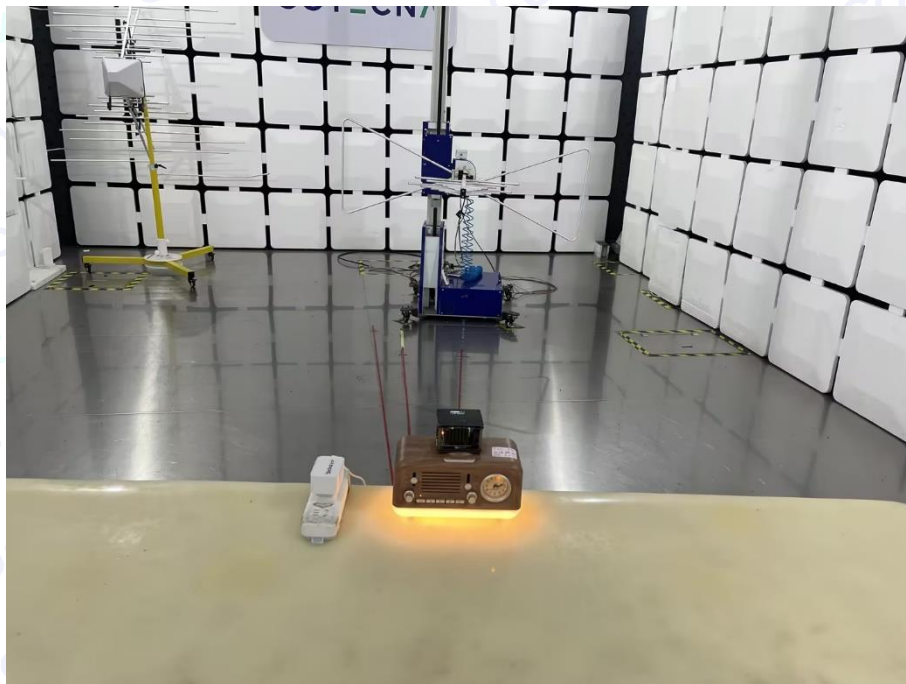
Photo of Setup for Radiated Emission (30MHz~1GHz)-WPT
