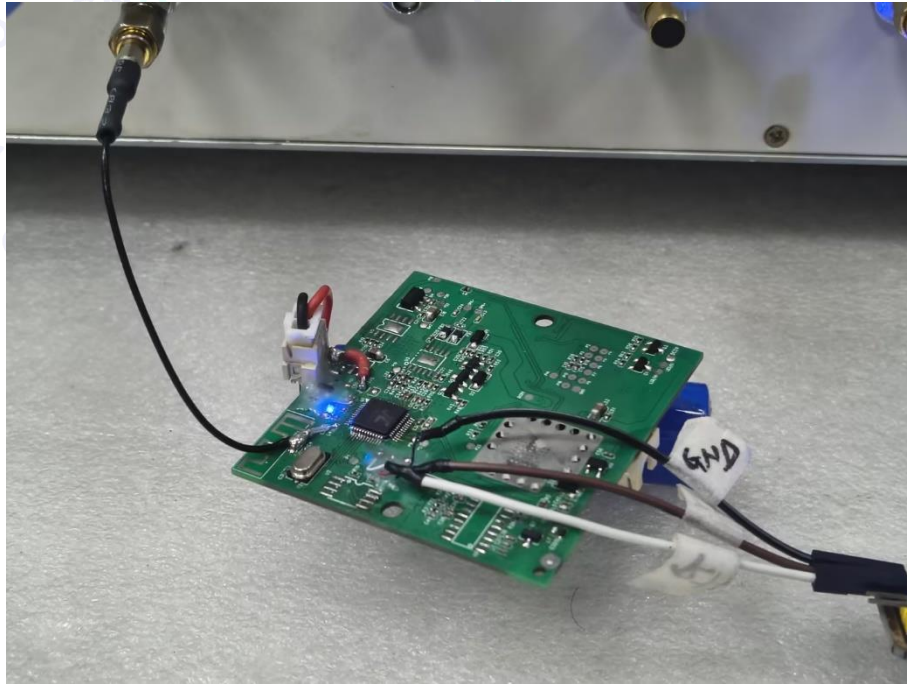
Photo of Setup for Conducted Emission(AC POWER)-WPT
