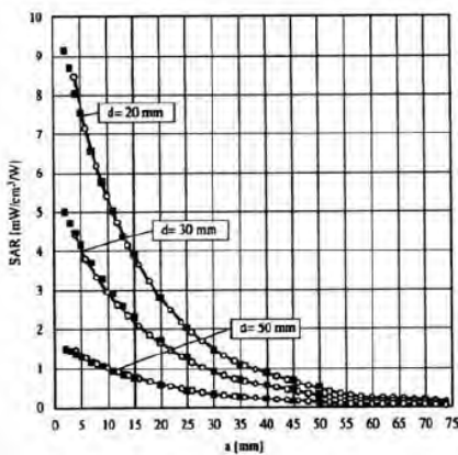
Figure 3.3.2 E-Field and Temperature Measurements at 900 MHz
