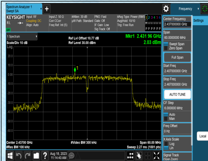
11N40SISO-Ant1-2437-0~Reference
