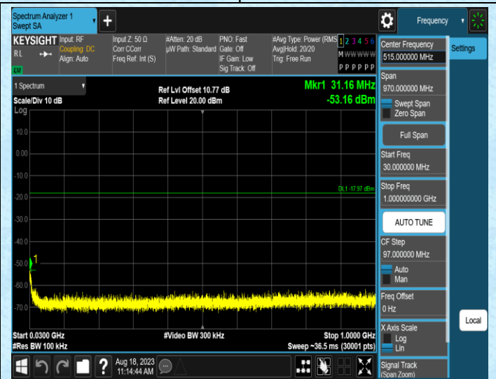
11N40SISO-Ant1-2437-30~1000
