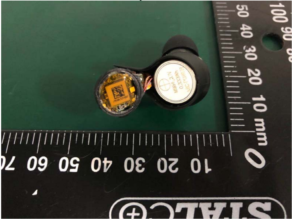
Internal Photos M/N: Epic Air ANC
