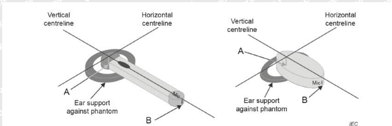
Figure 18 – An alternative form factor DUT with reference points and reference lines
