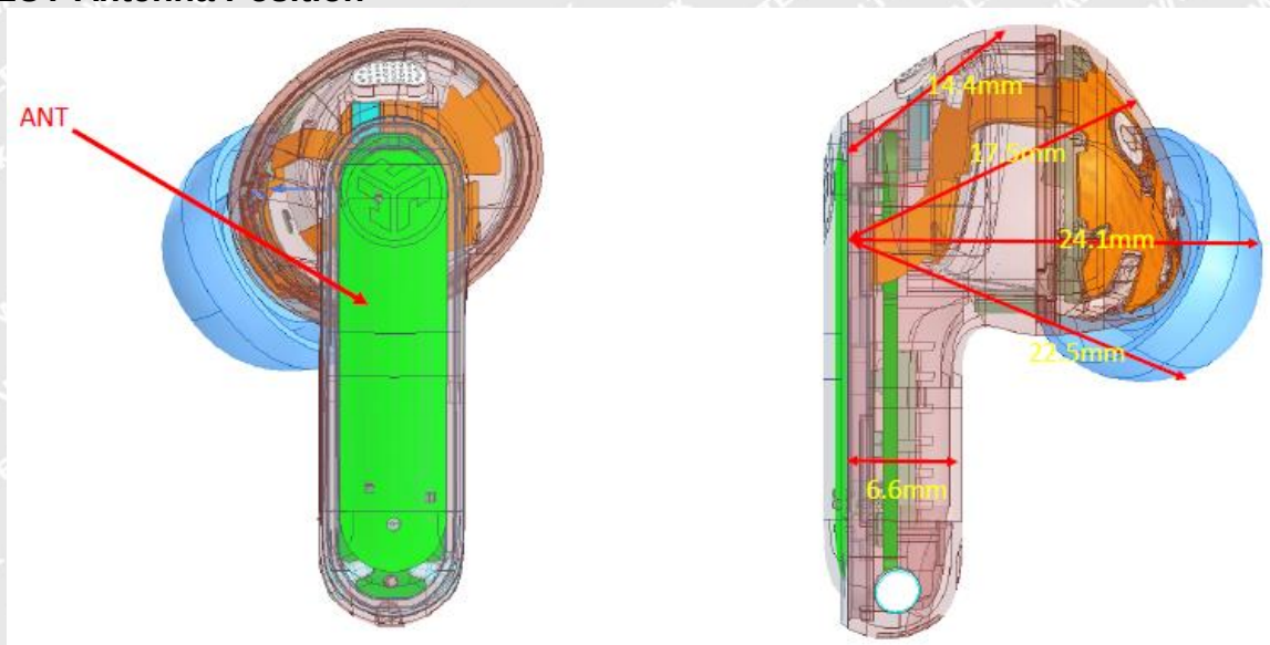
Fig 7.2 Block Diagram for EUT Antenna Position
