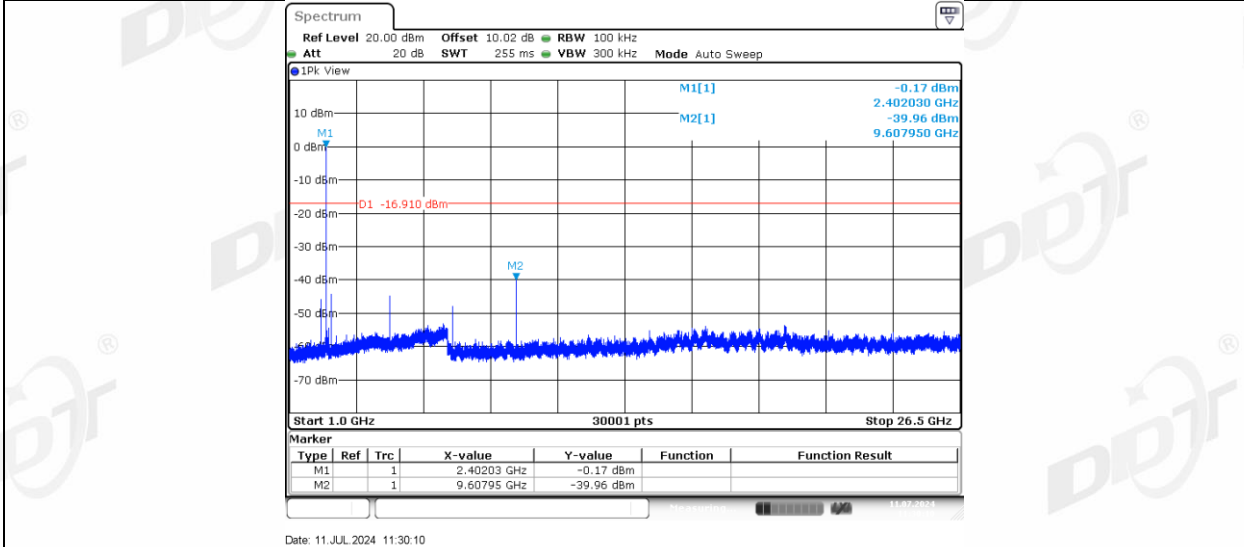
2DH5_Right side_2402_0~Reference
