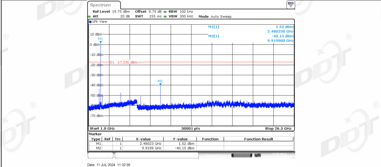
2DH5 Right side 2480 0~Reference
