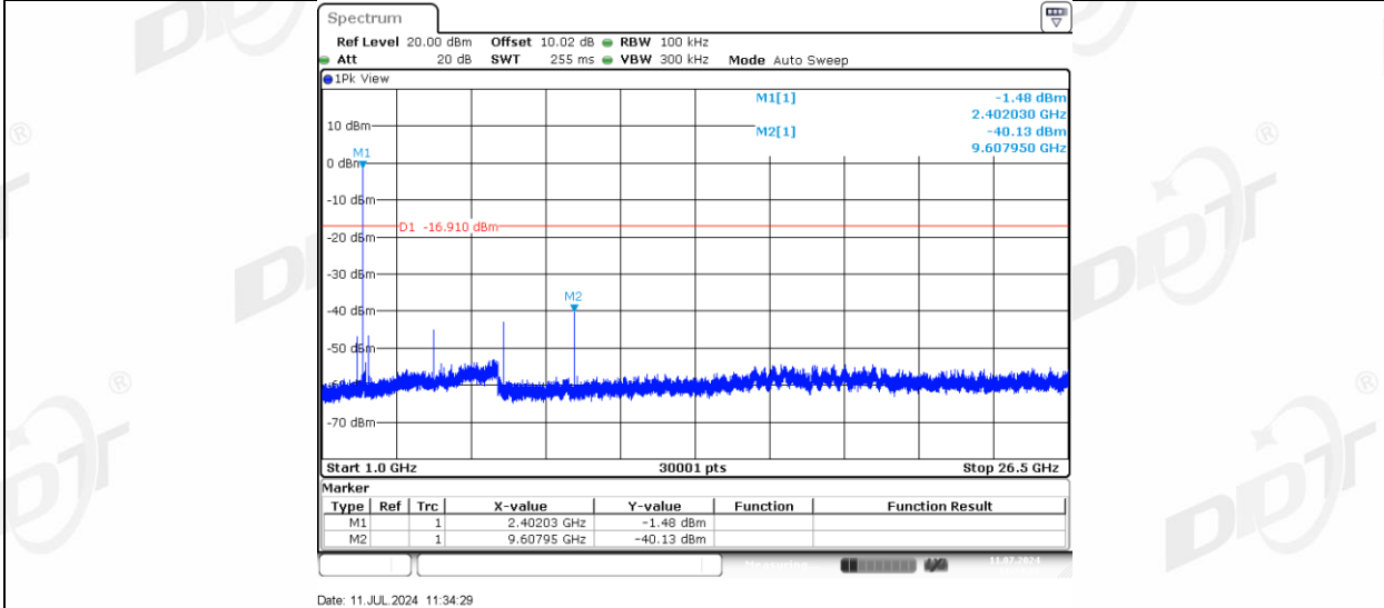
3DH5 Right side 2402 0~Reference
