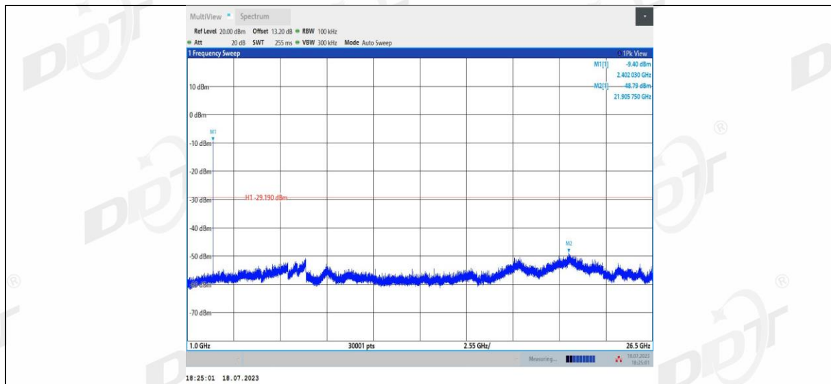
2DH5_Ant1_2441_0~Reference
