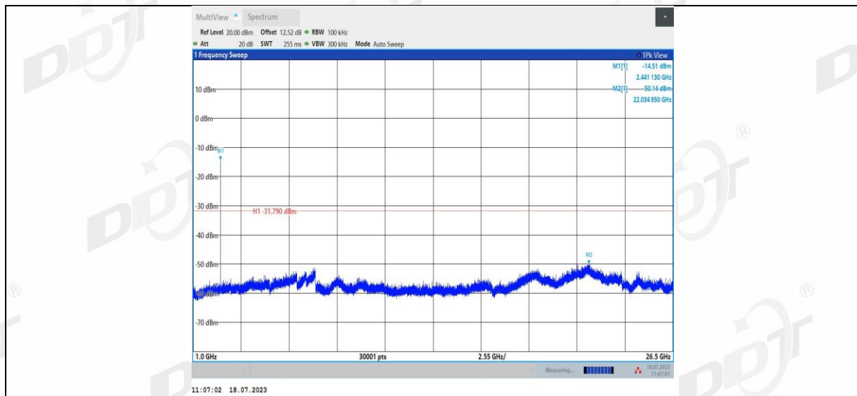
2DH5_Ant1_2480_0~Reference
