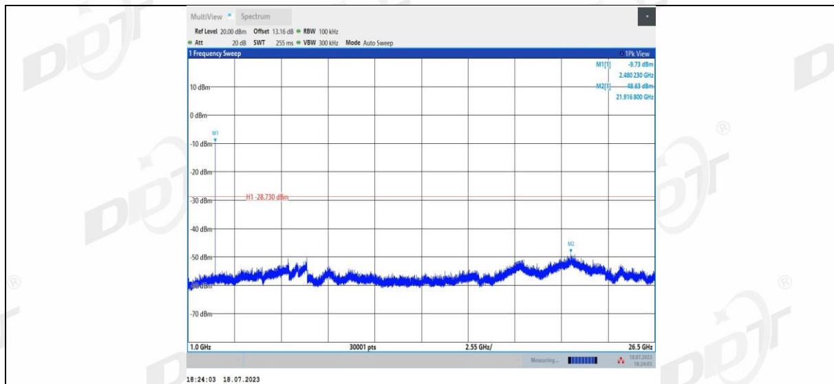
2DH5_Ant1_2402_0~Reference
