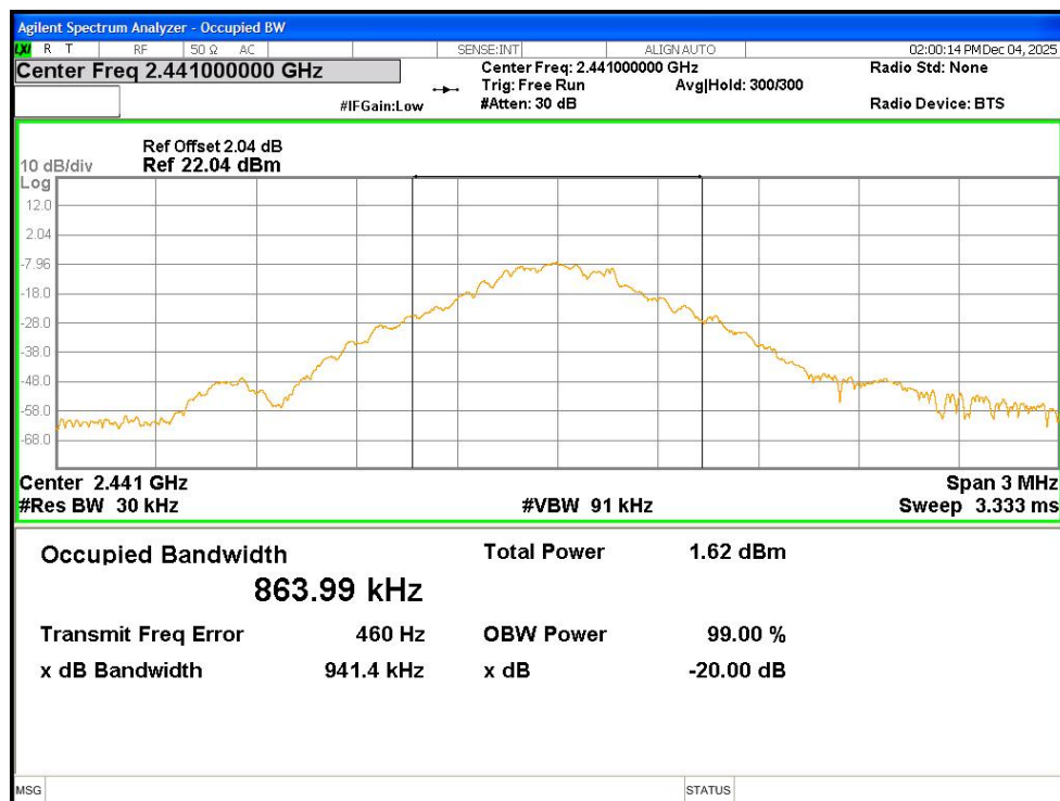
OBW NVNT 2.4G 2441MHz Ant1
