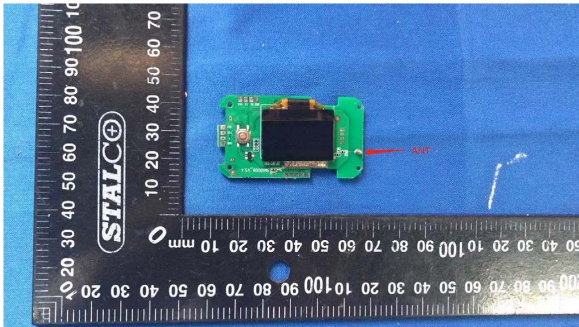
(2) Antenna Photo
