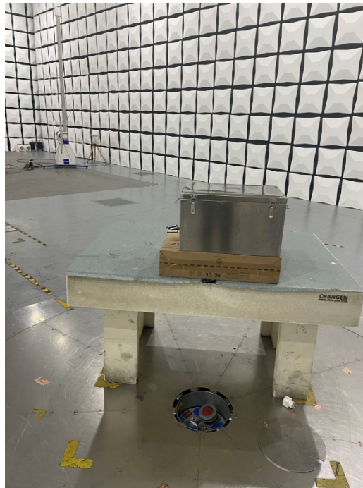
(2) Radiated spurious emission Test Setup(30MHz~1GHz)
