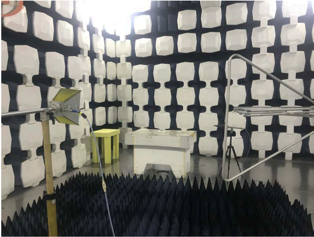
(2) Radiated spurious emission Test Setup(1GHz~18GHz)
