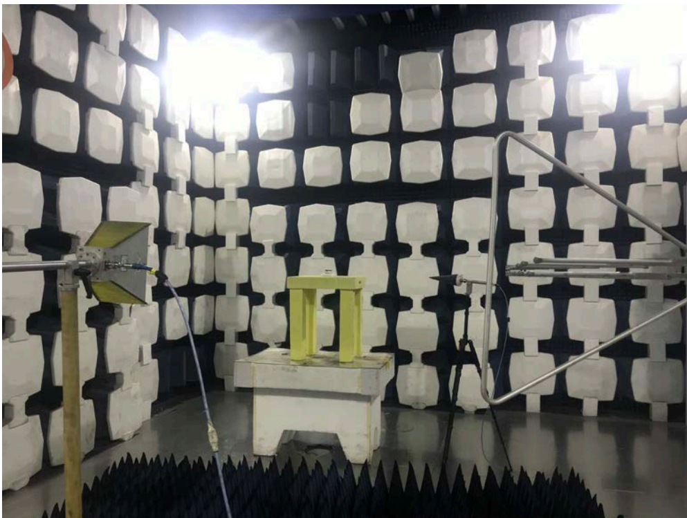
(2) Radiated spurious emission Test Setup(1GHz~18GHz)
