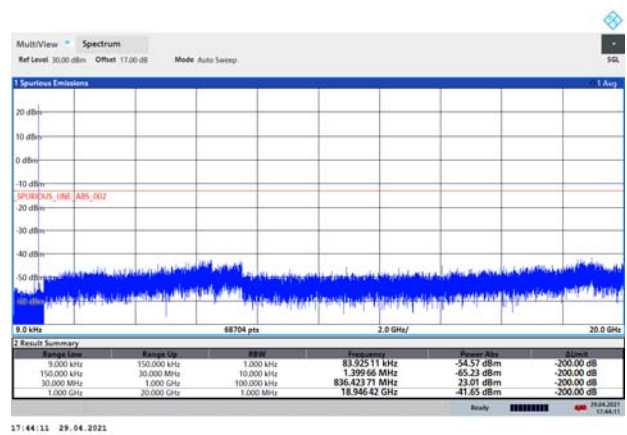
NB-IoT Band 5 CH-Middle 9kHz-20GHz
