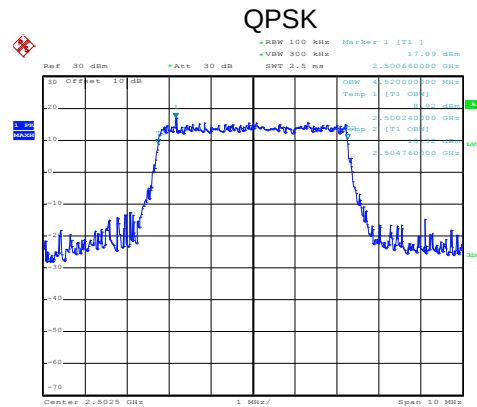
LTE Band 7: 99% Occupy bandwidth BW: 5MHz
