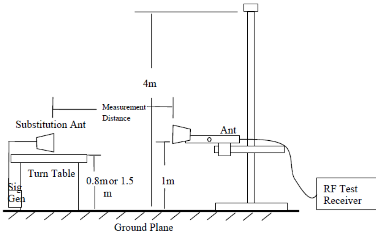
Figure 7—Substitution method set-up for radiated emission
