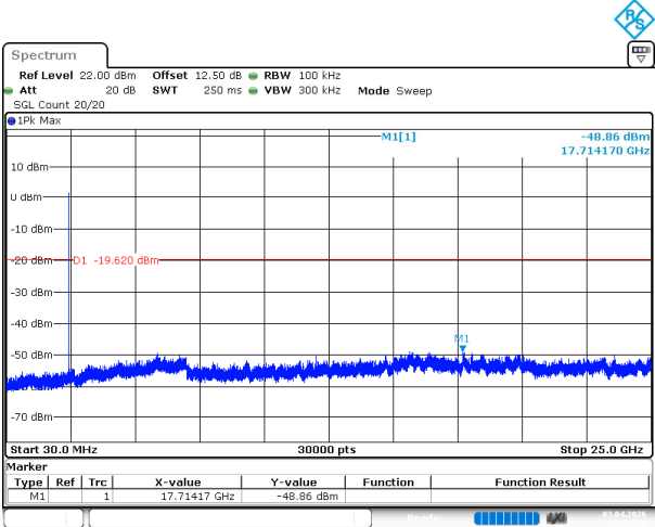
BDR_DH1_Middle
