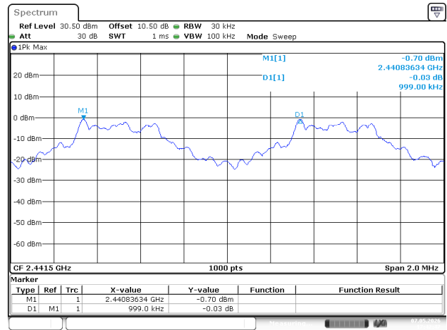
DH1_Middle
