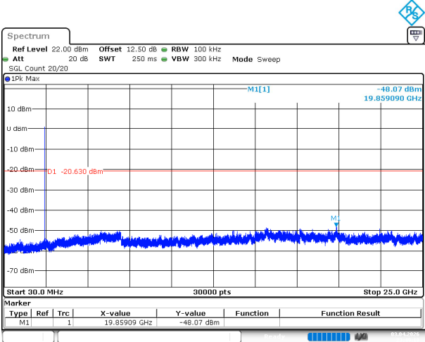
2EDR_2DH1_Middle
