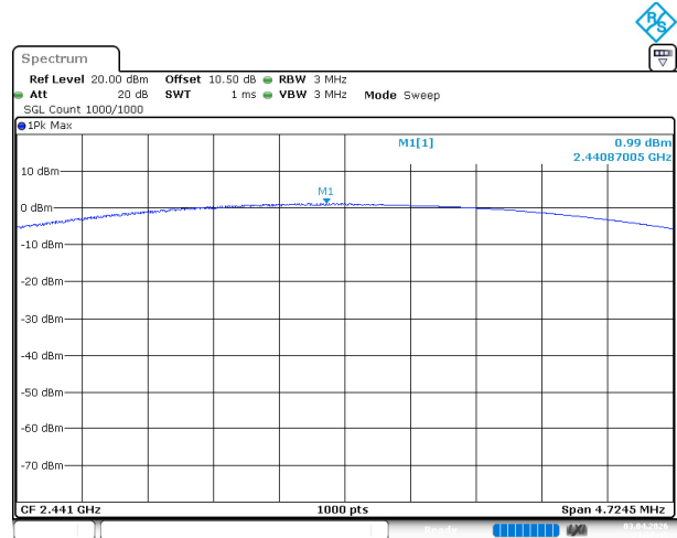
BDR_DH1_Middle
