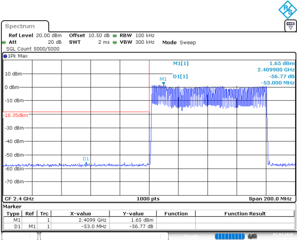
BDR_DH1_Hopping_Lower
