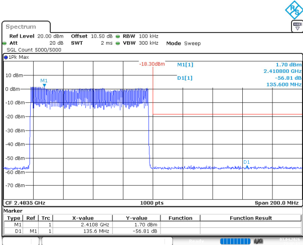
BDR_DH1_Hopping_Upper
