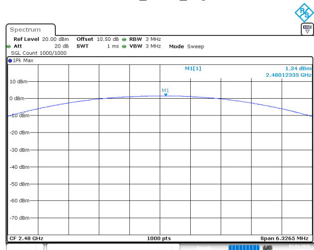
2EDR_2DH1_High
