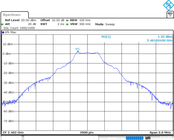
BDR_DH1_Low
