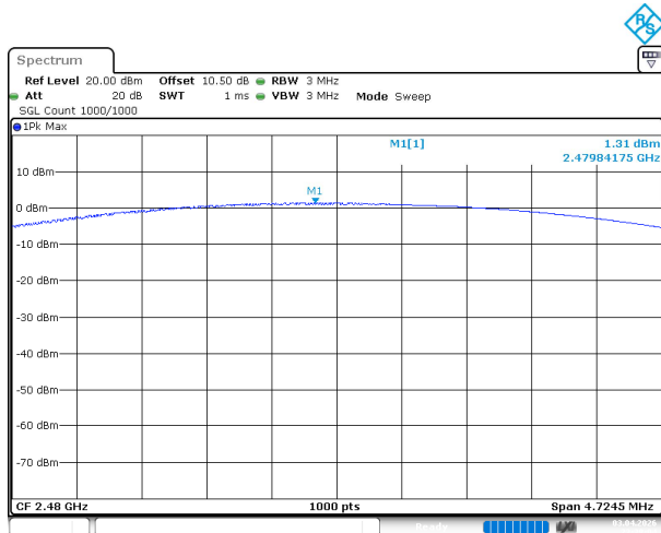
BDR_DH1_High
