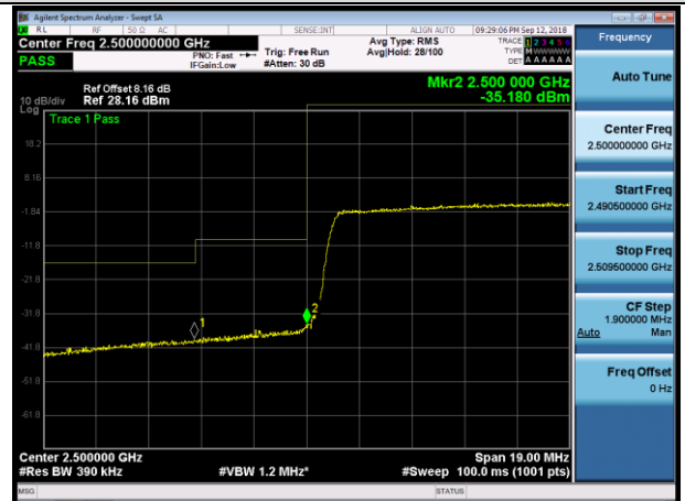
LCH_16QAM_100RB#0
