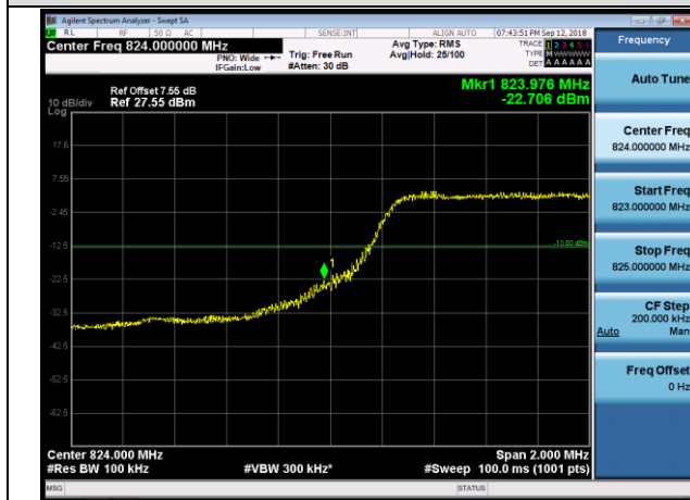
LCH_QPSK_25RB#0
