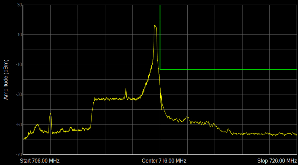
Band17 QPSK BW=5MHz Channel=23825 RB Size=1 Position=#Max
