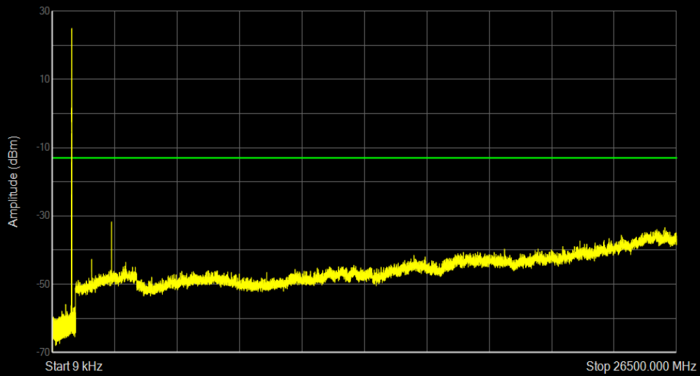
Band5 QAM16 BW=5MHz Channel=20625 RB Size=1 Position=#0
