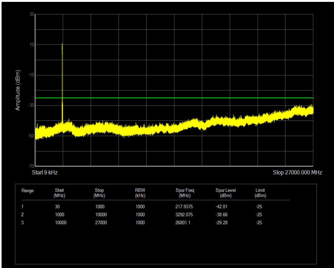
Band41(2593-2650) 16QAM BW=15MHz Channel=40695 RB Size=75 Position=#0
