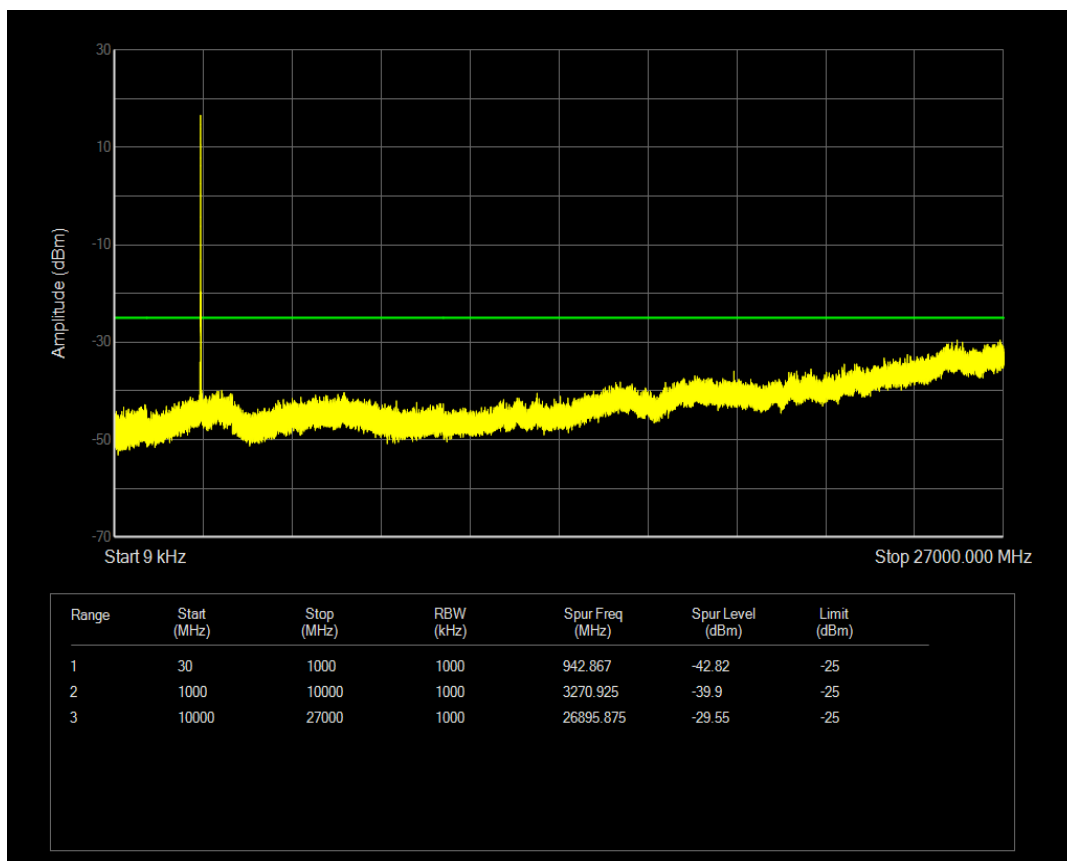
Band41(2593-2650) QPSK BW=20MHz Channel=41090 RB Size=1 Position=#Max
