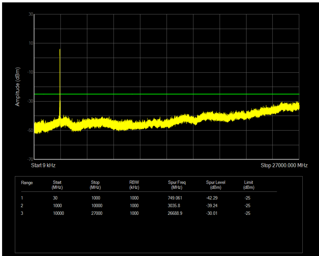
Band41(2593-2650) 16QAM BW=5MHz Channel=40645 RB Size=25 Position=#0
