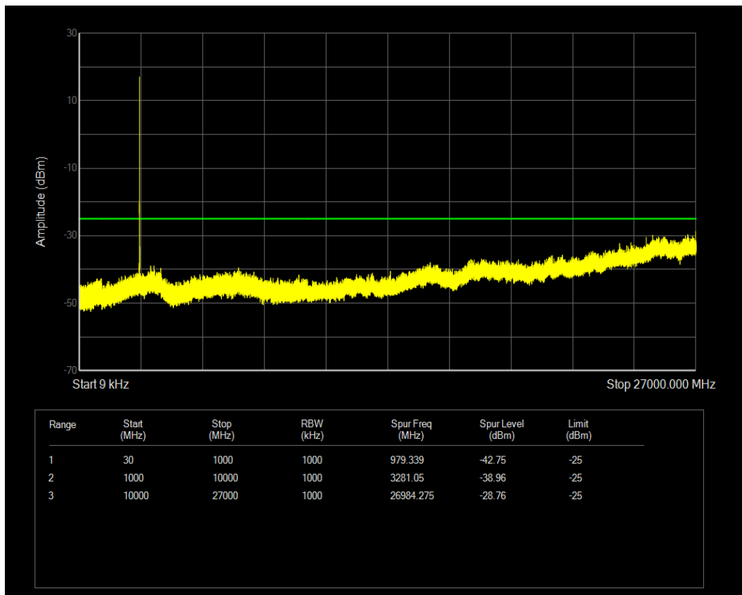
Band41(2593-2650) 16QAM BW=5MHz Channel=41165 RB Size=1 Position=#0
