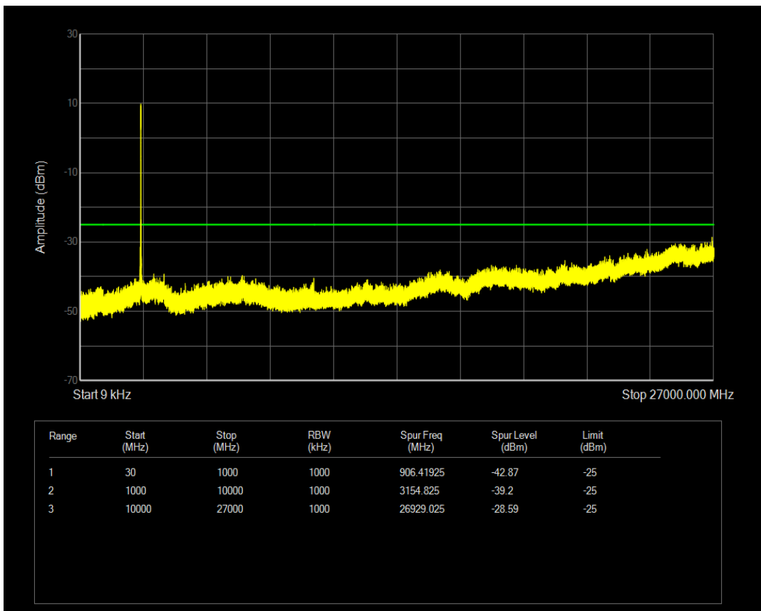
Band41(2593-2650) 16QAM BW=20MHz Channel=40720 RB Size=100 Position=#0
