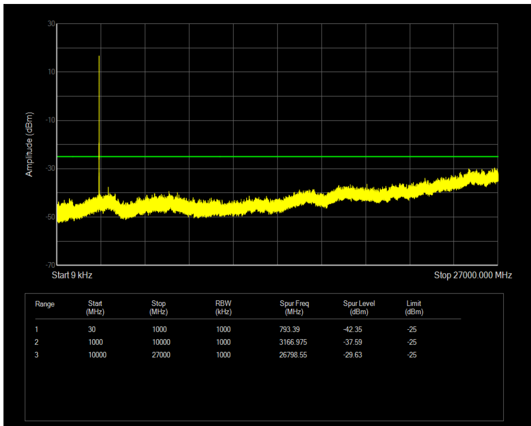
Band41(2593-2650) QPSK BW=15MHz Channel=41115 RB Size=1 Position=#0
