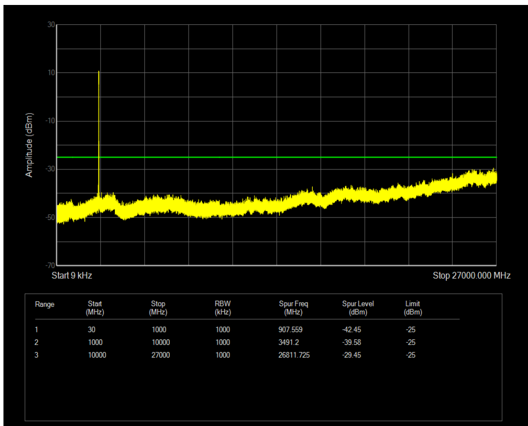
Band41(2593-2650) 16QAM BW=5MHz Channel=41165 RB Size=25 Position=#0
