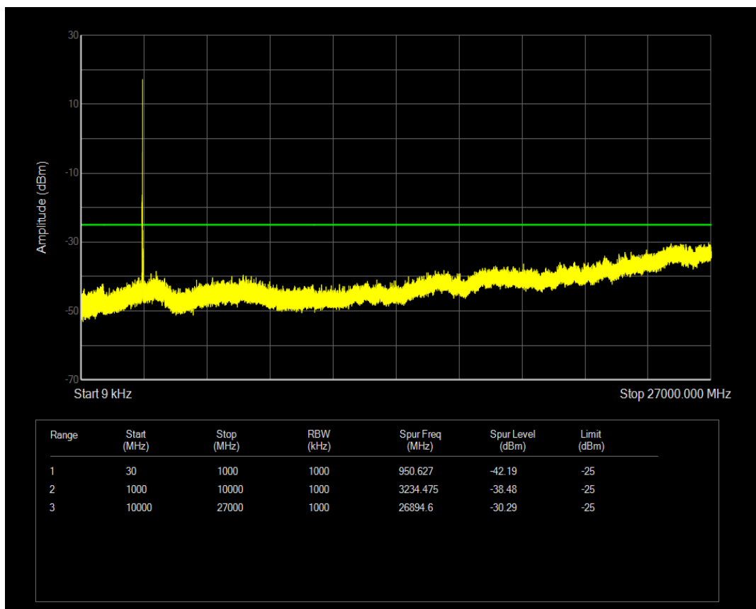
Band41(2593-2650) 16QAM BW=20MHz Channel=41090 RB Size=1 Position=#0
