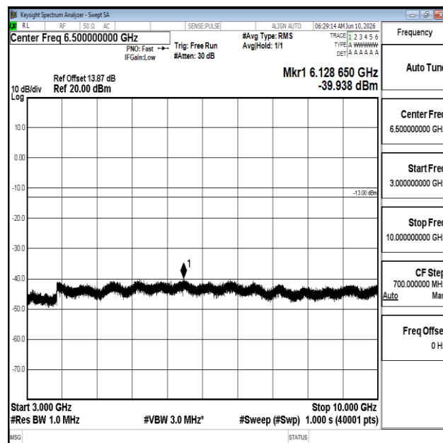
Band17-10MHz-16QAM-23800-50RB#0-3000~10000-PASS
