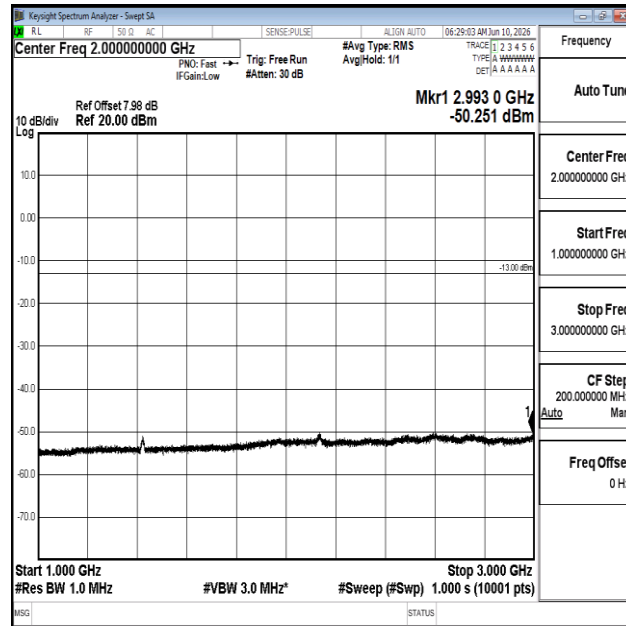
Band17-10MHz-16QAM-23800-50RB#0-1000~3000-PASS
