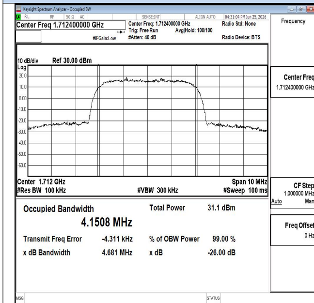
Channel 1312 / 1712.4 MHz
