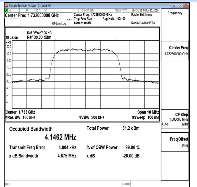
Channel 1413 / 1732.6 MHz
