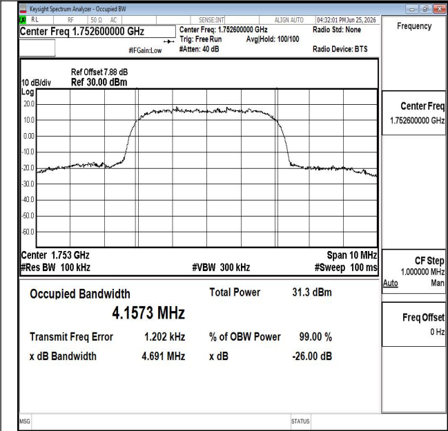
Channel 1513 / 1752.6 MHz
