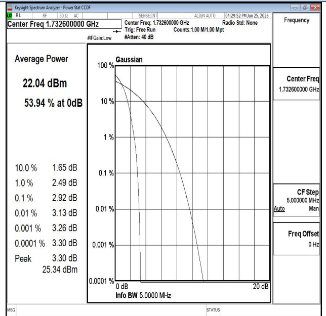
Channel 1413 / 1732.6 MHz
